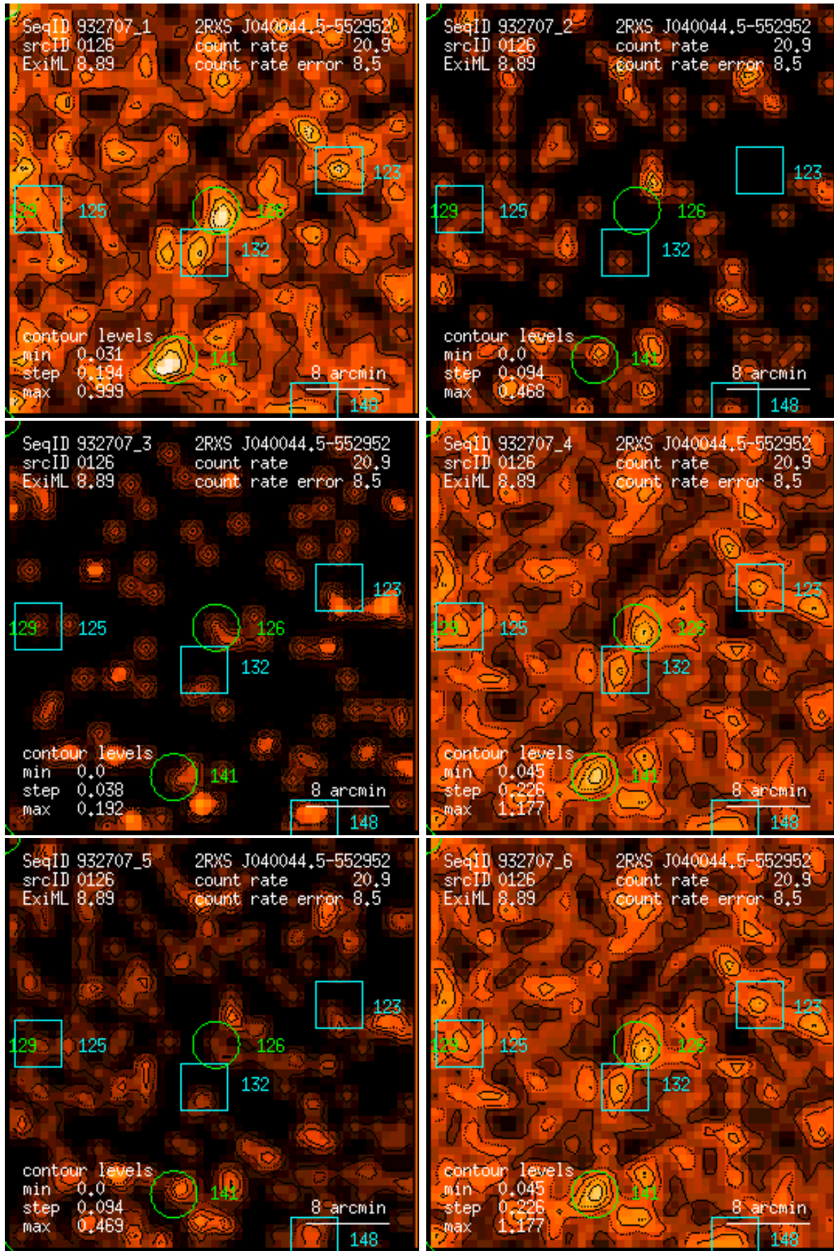
Figure 126: RASS 932707: detection 0126: band rate images, Gaussian filter: (1) PSPC channels 11 – 41, (2) 52 – 90, (3) 91 – 201, (4) 11 – 235, (5) 52 – 201, (6) 11 – 201. Broad band rates in counts/ks. Band rate contour levels in counts/ks/arcmin 2 .
