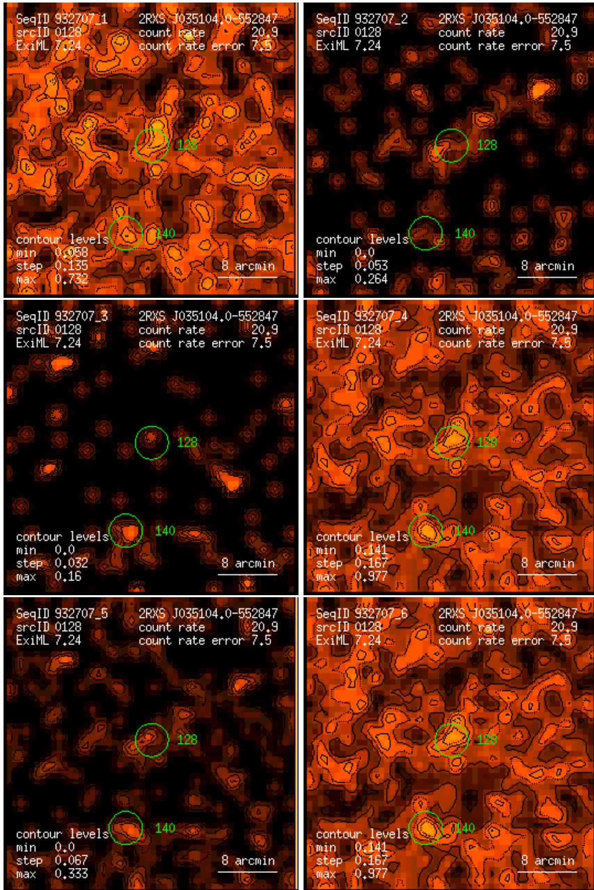
Figure 128: RASS 932707: detection 0128: band rate images, Gaussian filter: (1) PSPC channels 11 – 41, (2) 52 – 90, (3) 91 – 201, (4) 11 – 235, (5) 52 – 201, (6) 11 – 201. Broad band rates in counts/ks. Band rate contour levels in counts/ks/arcmin 2 .
