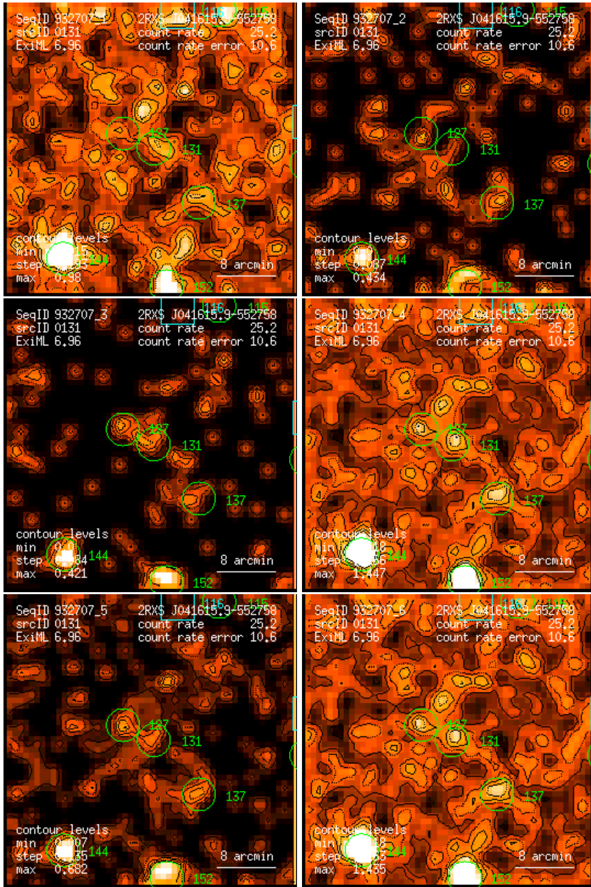
Figure 131: RASS 932707: detection 0131: band rate images, Gaussian filter: (1) PSPC channels 11 – 41, (2) 52 – 90, (3) 91 – 201, (4) 11 – 235, (5) 52 – 201, (6) 11 – 201. Broad band rates in counts/ks. Band rate contour levels in counts/ks/arcmin 2 .
