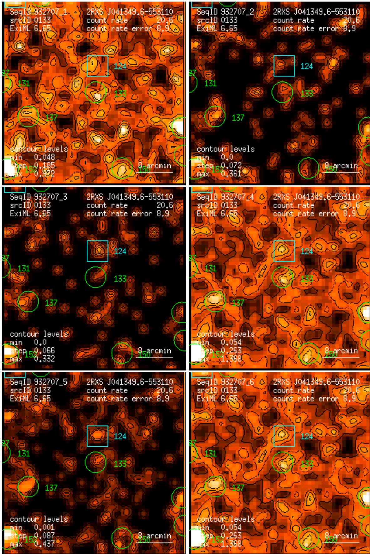
Figure 133: RASS 932707: detection 0133: band rate images, Gaussian filter: (1) PSPC channels 11 – 41, (2) 52 – 90, (3) 91 – 201, (4) 11 – 235, (5) 52 – 201, (6) 11 – 201. Broad band rates in counts/ks. Band rate contour levels in counts/ks/arcmin 2 .
