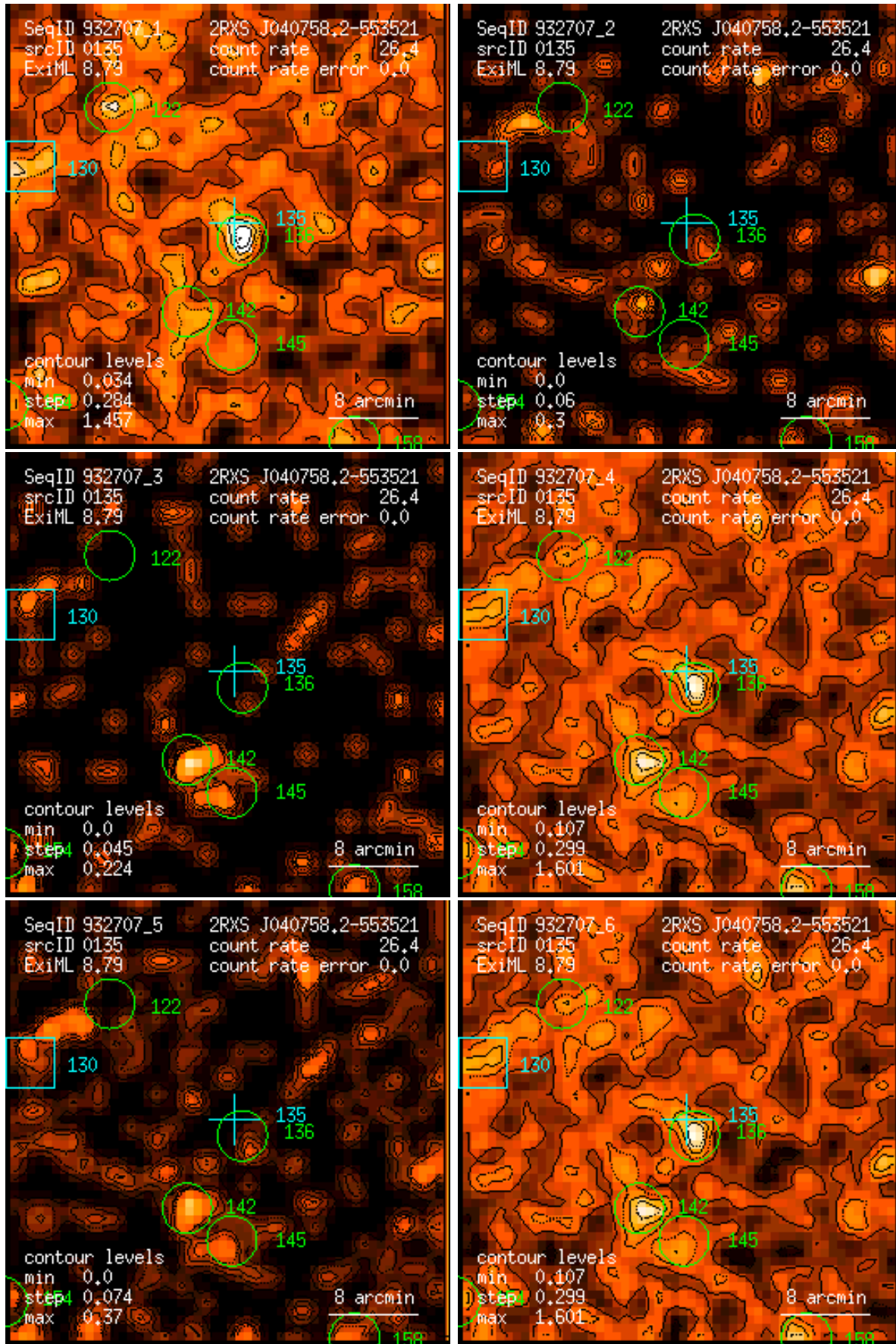
Figure 135: RASS 932707: detection 0135: band rate images, Gaussian filter: (1) PSPC channels 11 – 41, (2) 52 – 90, (3) 91 – 201, (4) 11 – 235, (5) 52 – 201, (6) 11 – 201. Broad band rates in counts/ks. Band rate contour levels in counts/ks/arcmin 2 .
