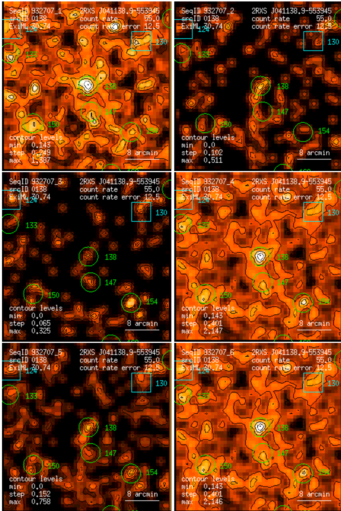
Figure 138: RASS 932707: detection 0138: band rate images, Gaussian filter: (1) PSPC channels 11 – 41, (2) 52 – 90, (3) 91 – 201, (4) 11 – 235, (5) 52 – 201, (6) 11 – 201. Broad band rates in counts/ks. Band rate contour levels in counts/ks/arcmin 2 .
