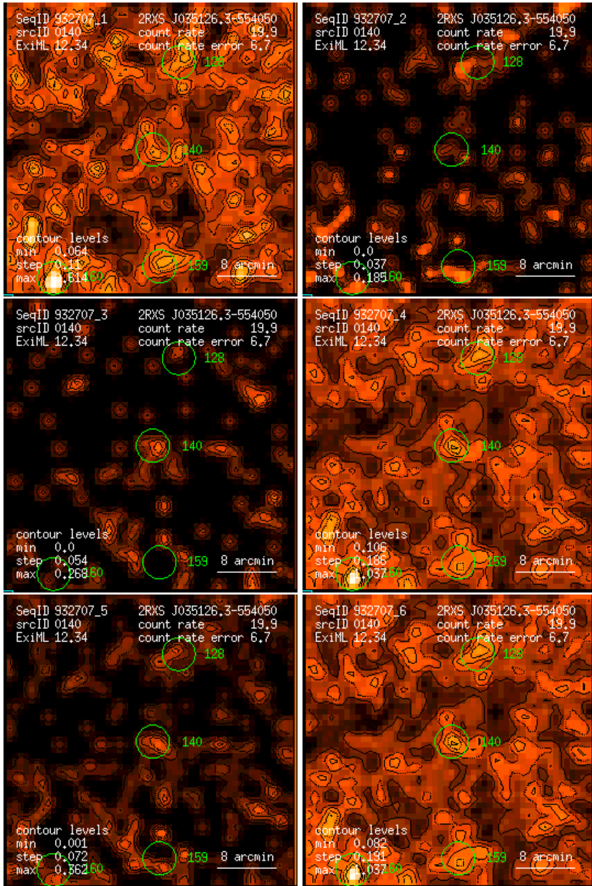
Figure 140: RASS 932707: detection 0140: band rate images, Gaussian filter: (1) PSPC channels 11 – 41, (2) 52 – 90, (3) 91 – 201, (4) 11 – 235, (5) 52 – 201, (6) 11 – 201. Broad band rates in counts/ks. Band rate contour levels in counts/ks/arcmin 2 .
