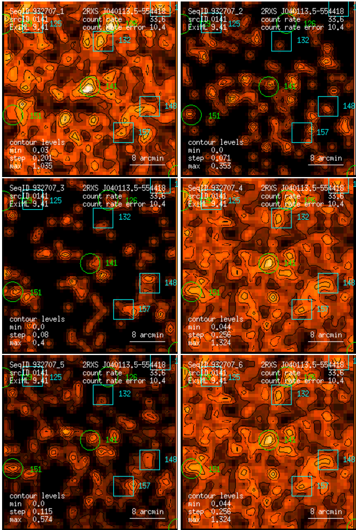
Figure 141: RASS 932707: detection 0141: band rate images, Gaussian filter: (1) PSPC channels 11 – 41, (2) 52 – 90, (3) 91 – 201, (4) 11 – 235, (5) 52 – 201, (6) 11 – 201. Broad band rates in counts/ks. Band rate contour levels in counts/ks/arcmin 2 .
