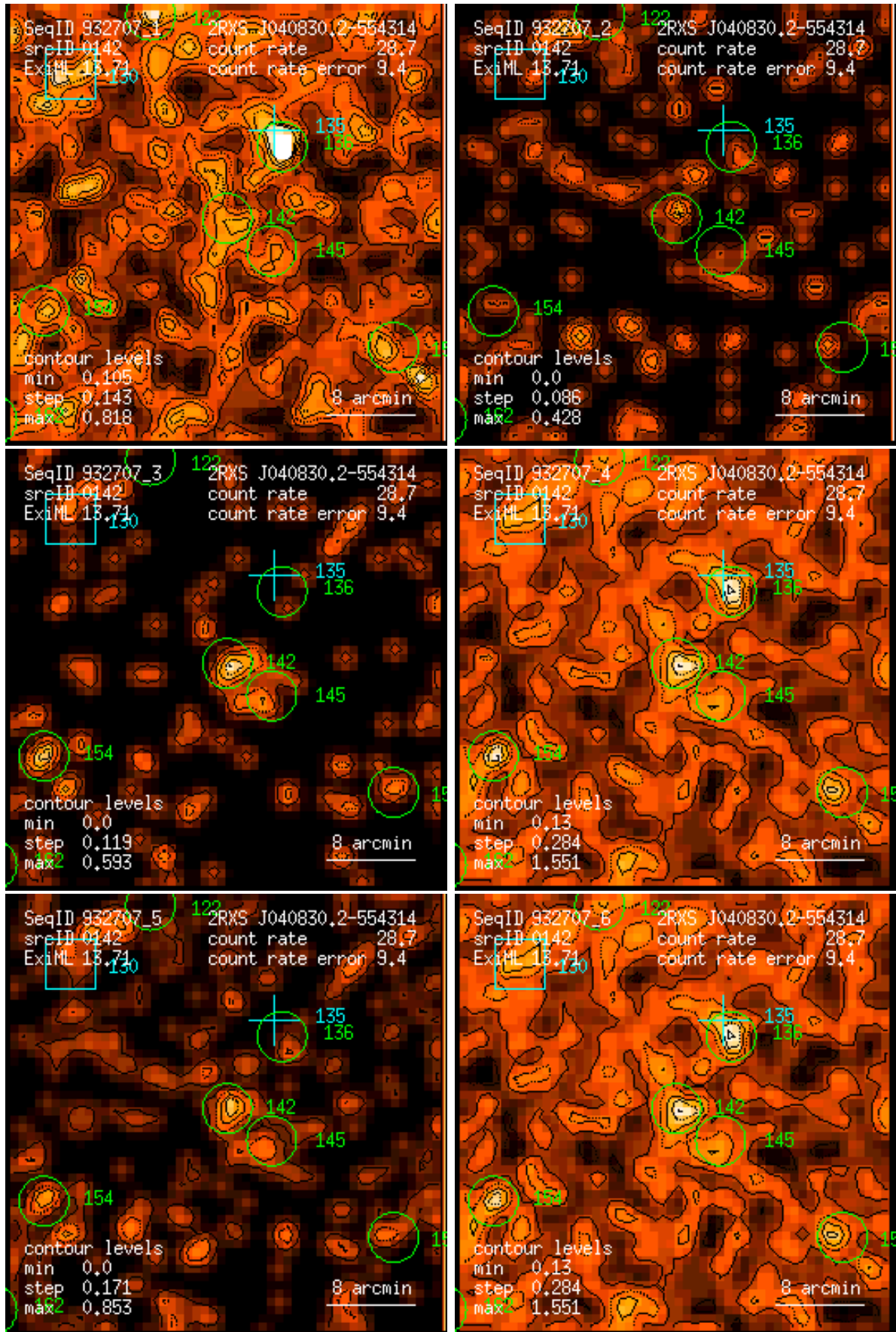
Figure 142: RASS 932707: detection 0142: band rate images, Gaussian filter: (1) PSPC channels 11 – 41, (2) 52 – 90, (3) 91 – 201, (4) 11 – 235, (5) 52 – 201, (6) 11 – 201. Broad band rates in counts/ks. Band rate contour levels in counts/ks/arcmin 2 .
