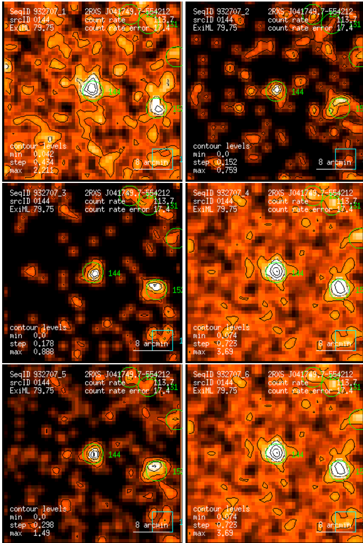
Figure 144: RASS 932707: detection 0144: band rate images, Gaussian filter: (1) PSPC channels 11 – 41, (2) 52 – 90, (3) 91 – 201, (4) 11 – 235, (5) 52 – 201, (6) 11 – 201. Broad band rates in counts/ks. Band rate contour levels in counts/ks/arcmin 2 .
