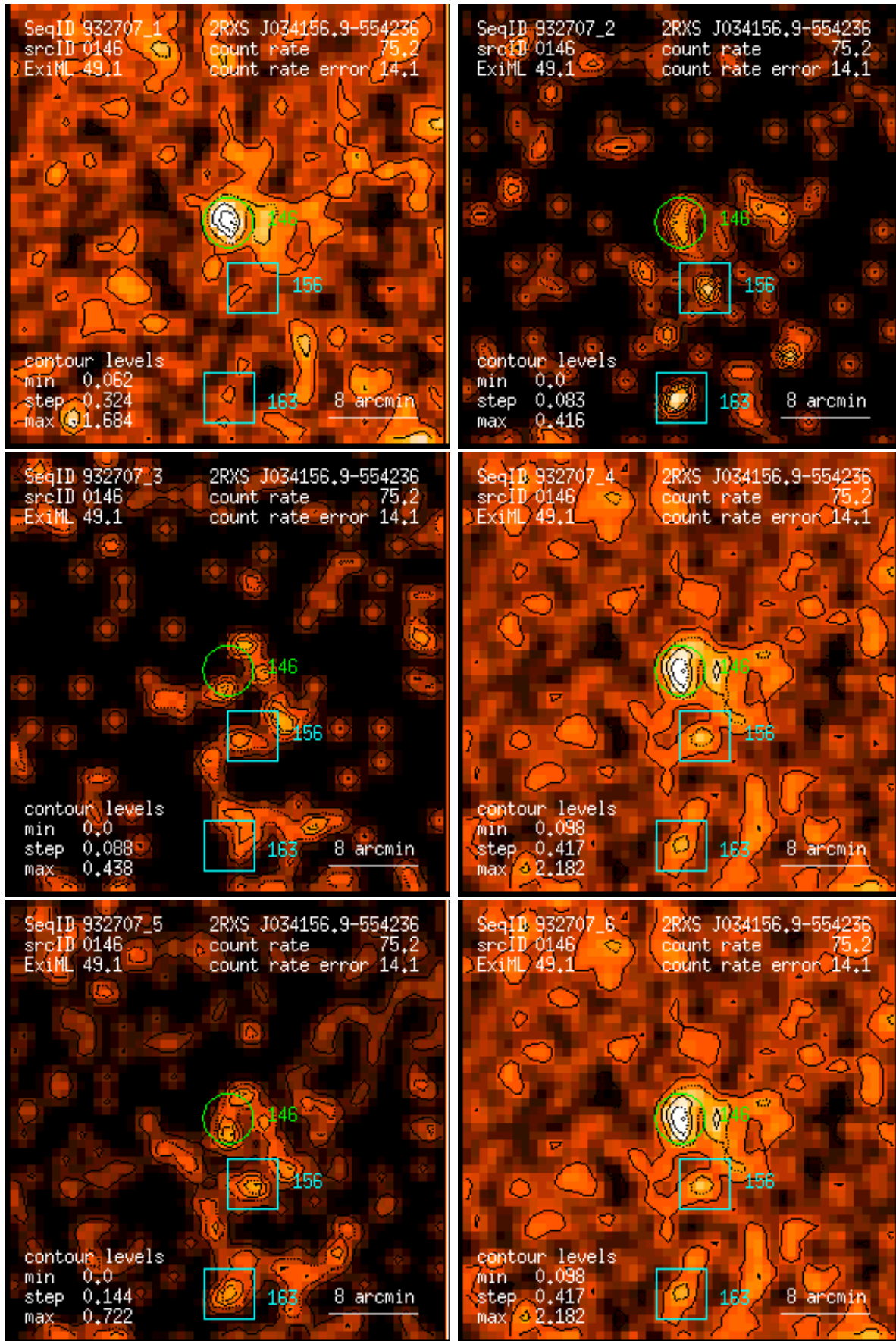
Figure 146: RASS 932707: detection 0146: band rate images, Gaussian filter: (1) PSPC channels 11 – 41, (2) 52 – 90, (3) 91 – 201, (4) 11 – 235, (5) 52 – 201, (6) 11 – 201. Broad band rates in counts/ks. Band rate contour levels in counts/ks/arcmin 2 .
