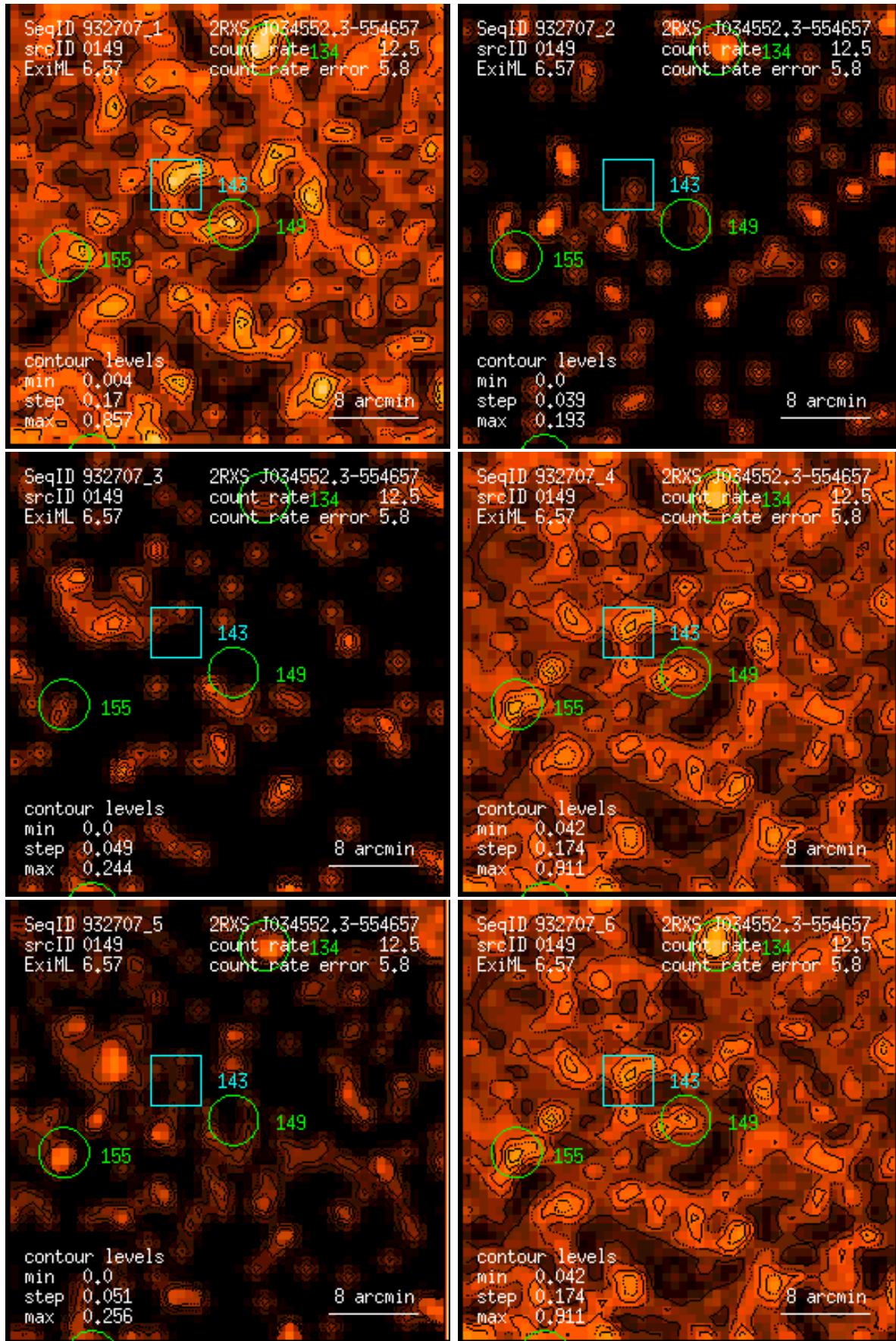
Figure 149: RASS 932707: detection 0149: band rate images, Gaussian filter: (1) PSPC channels 11 – 41, (2) 52 – 90, (3) 91 – 201, (4) 11 – 235, (5) 52 – 201, (6) 11 – 201. Broad band rates in counts/ks. Band rate contour levels in counts/ks/arcmin 2 .
