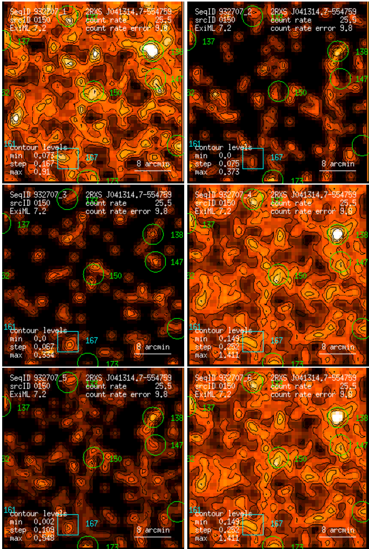
Figure 150: RASS 932707: detection 0150: band rate images, Gaussian filter: (1) PSPC channels 11 – 41, (2) 52 – 90, (3) 91 – 201, (4) 11 – 235, (5) 52 – 201, (6) 11 – 201. Broad band rates in counts/ks. Band rate contour levels in counts/ks/arcmin 2 .
