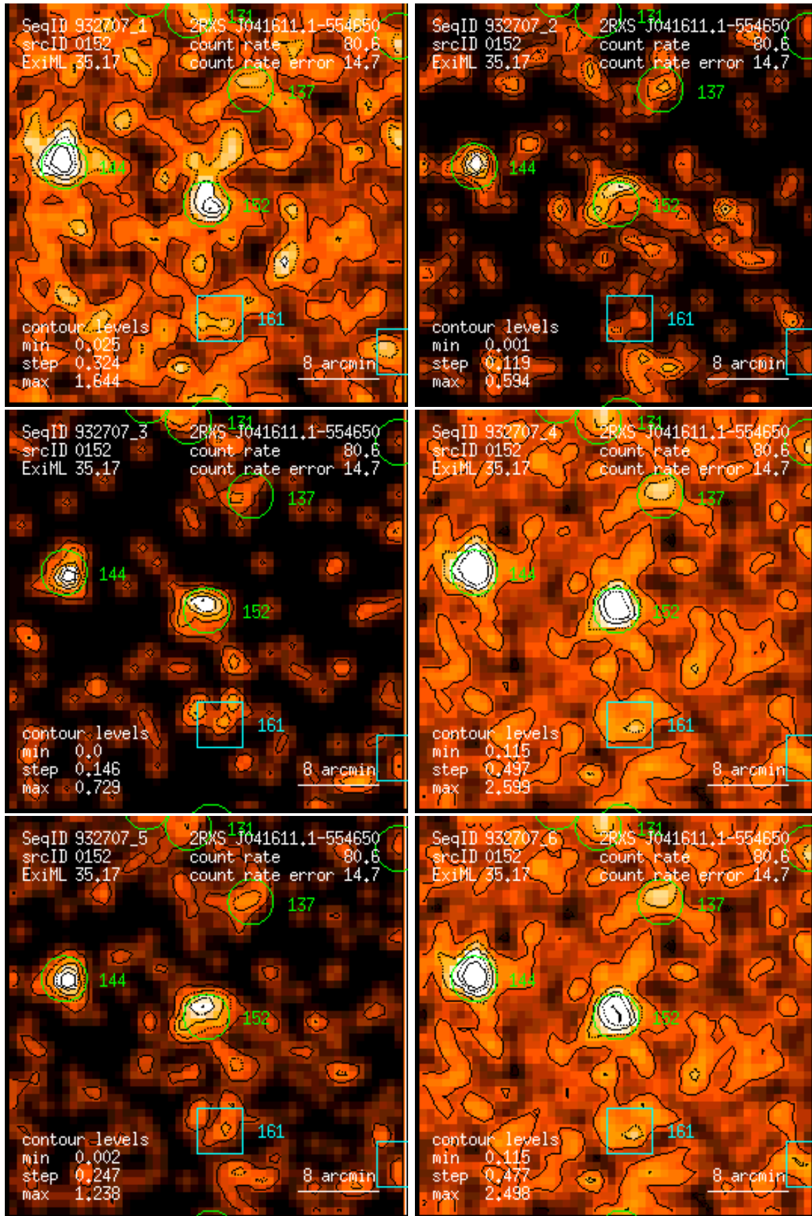
Figure 152: RASS 932707: detection 0152: band rate images, Gaussian filter: (1) PSPC channels 11 – 41, (2) 52 – 90, (3) 91 – 201, (4) 11 – 235, (5) 52 – 201, (6) 11 – 201. Broad band rates in counts/ks. Band rate contour levels in counts/ks/arcmin 2 .
