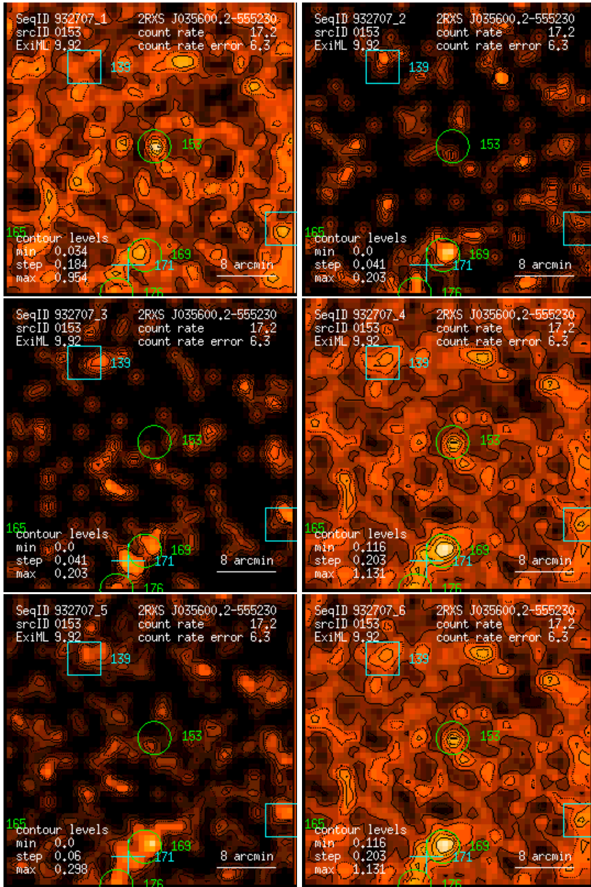
Figure 153: RASS 932707: detection 0153: band rate images, Gaussian filter: (1) PSPC channels 11 – 41, (2) 52 – 90, (3) 91 – 201, (4) 11 – 235, (5) 52 – 201, (6) 11 – 201. Broad band rates in counts/ks. Band rate contour levels in counts/ks/arcmin 2 .
