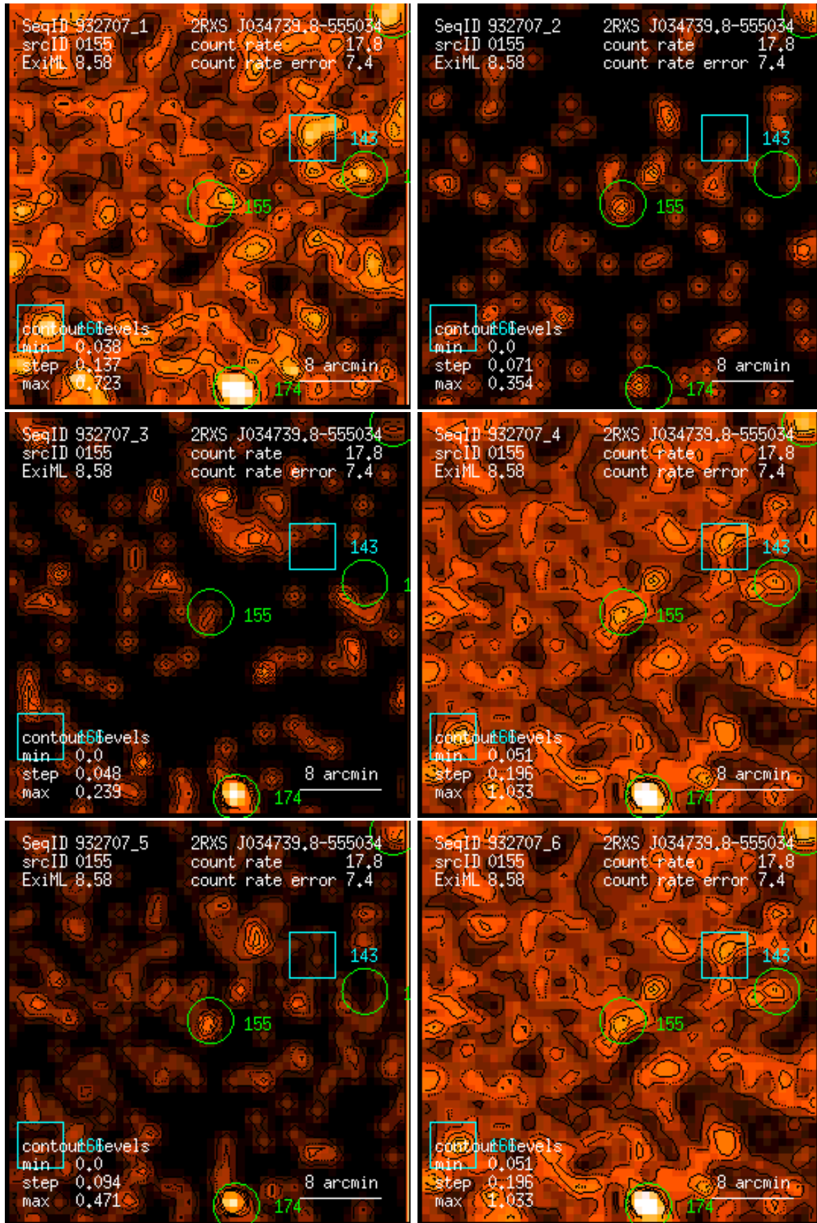
Figure 155: RASS 932707: detection 0155: band rate images, Gaussian filter: (1) PSPC channels 11 – 41, (2) 52 – 90, (3) 91 – 201, (4) 11 – 235, (5) 52 – 201, (6) 11 – 201. Broad band rates in counts/ks. Band rate contour levels in counts/ks/arcmin 2 .
