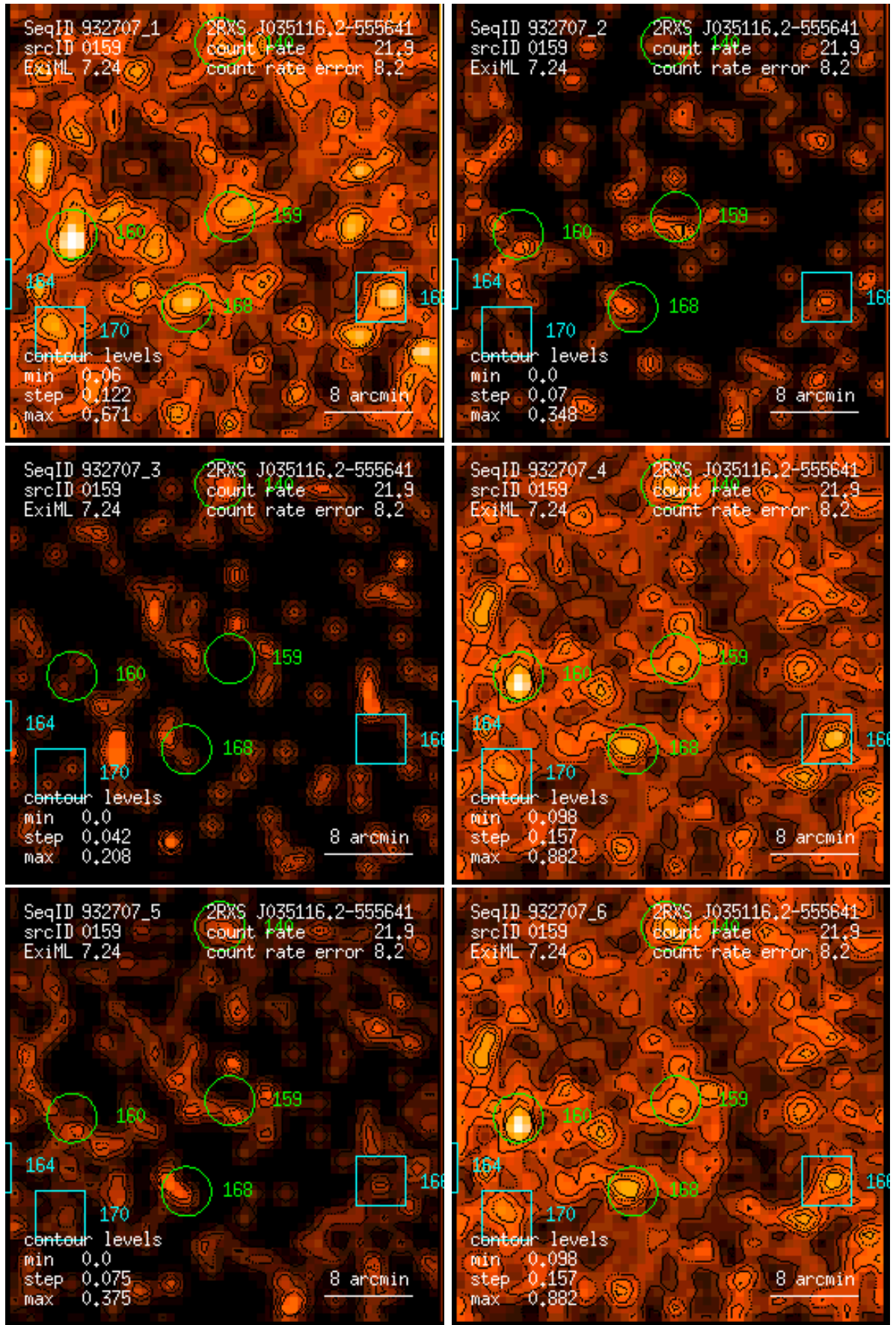
Figure 159: RASS 932707: detection 0159: band rate images, Gaussian filter: (1) PSPC channels 11 – 41, (2) 52 – 90, (3) 91 – 201, (4) 11 – 235, (5) 52 – 201, (6) 11 – 201. Broad band rates in counts/ks. Band rate contour levels in counts/ks/arcmin 2 .
