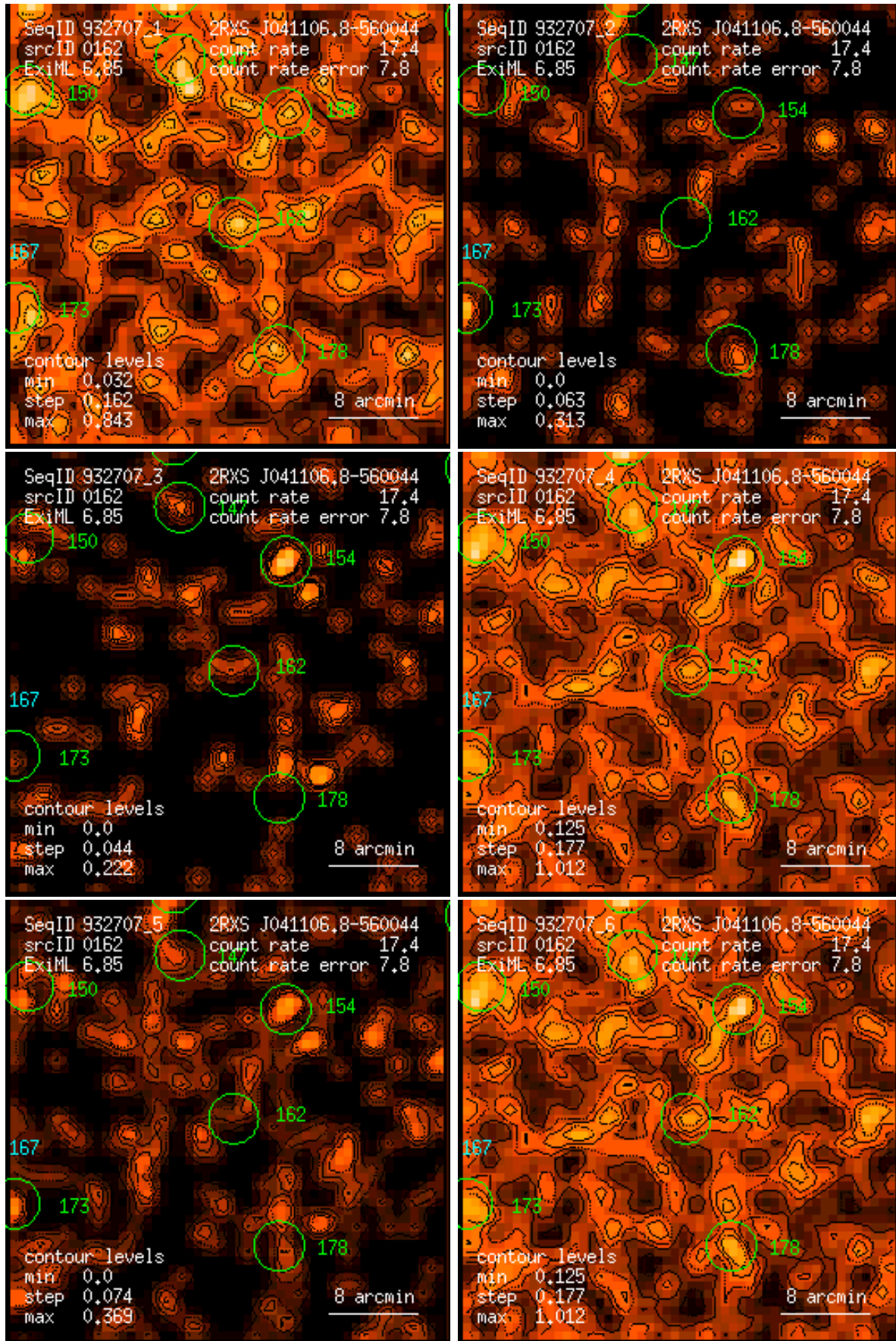
Figure 162: RASS 932707: detection 0162: band rate images, Gaussian filter: (1) PSPC channels 11 – 41, (2) 52 – 90, (3) 91 – 201, (4) 11 – 235, (5) 52 – 201, (6) 11 – 201. Broad band rates in counts/ks. Band rate contour levels in counts/ks/arcmin 2 .
