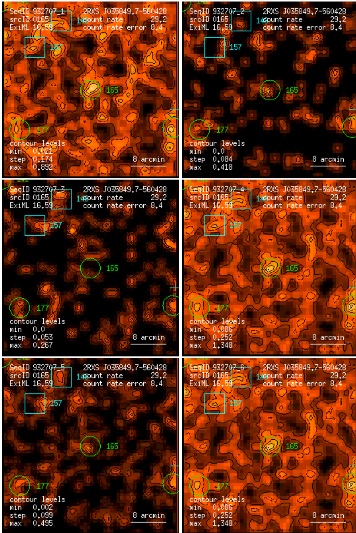
Figure 165: RASS 932707: detection 0165: band rate images, Gaussian filter: (1) PSPC channels 11 – 41, (2) 52 – 90, (3) 91 – 201, (4) 11 – 235, (5) 52 – 201, (6) 11 – 201. Broad band rates in counts/ks. Band rate contour levels in counts/ks/arcmin 2 .
