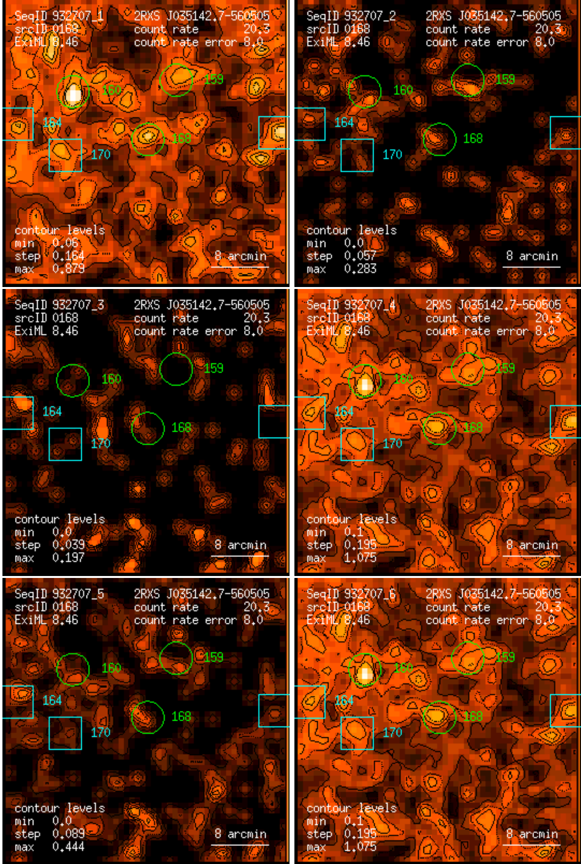
Figure 168: RASS 932707: detection 0168: band rate images, Gaussian filter: (1) PSPC channels 11 – 41, (2) 52 – 90, (3) 91 – 201, (4) 11 – 235, (5) 52 – 201, (6) 11 – 201. Broad band rates in counts/ks. Band rate contour levels in counts/ks/arcmin 2 .
