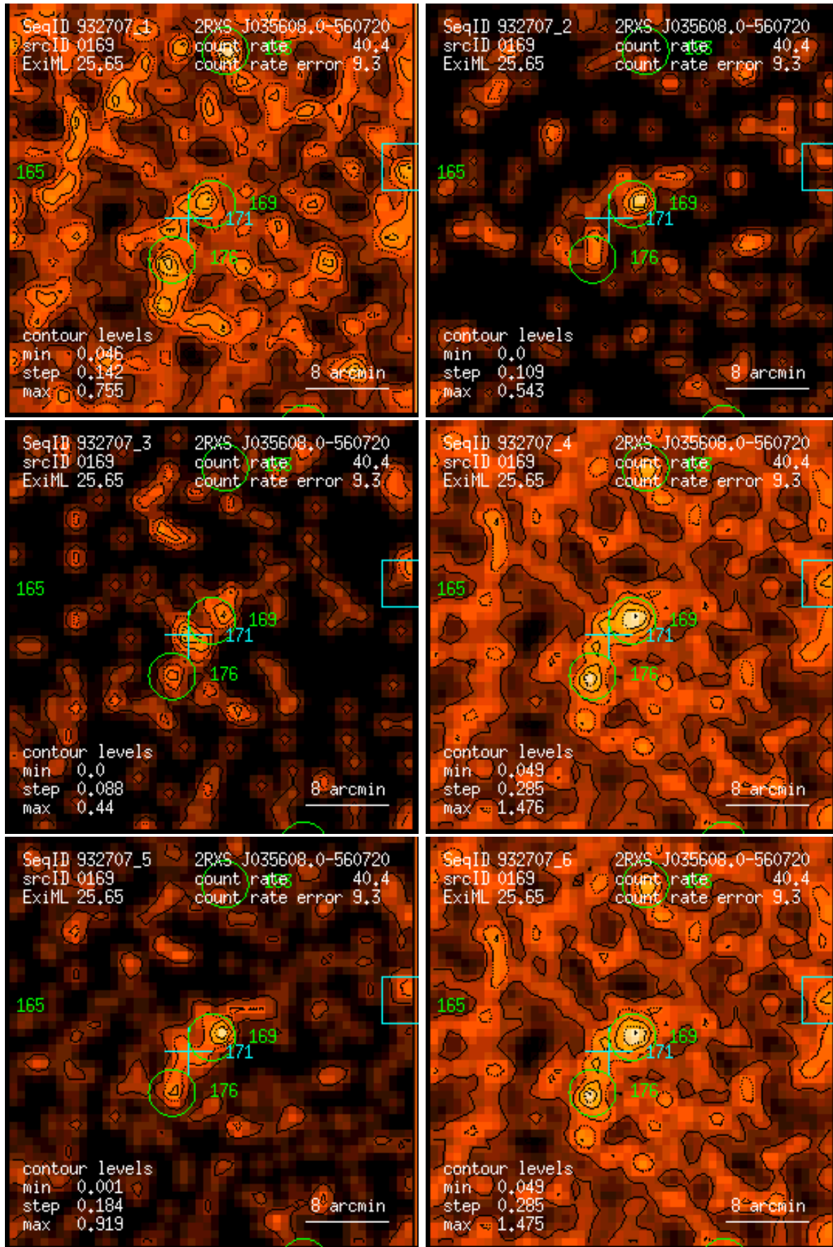
Figure 169: RASS 932707: detection 0169: band rate images, Gaussian filter: (1) PSPC channels 11 – 41, (2) 52 – 90, (3) 91 – 201, (4) 11 – 235, (5) 52 – 201, (6) 11 – 201. Broad band rates in counts/ks. Band rate contour levels in counts/ks/arcmin 2 .
