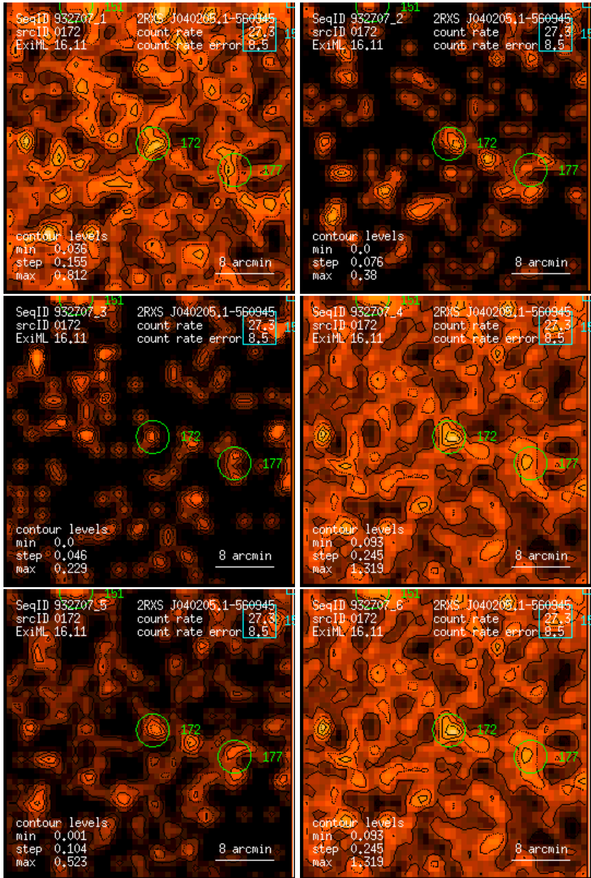
Figure 172: RASS 932707: detection 0172: band rate images, Gaussian filter: (1) PSPC channels 11 – 41, (2) 52 – 90, (3) 91 – 201, (4) 11 – 235, (5) 52 – 201, (6) 11 – 201. Broad band rates in counts/ks. Band rate contour levels in counts/ks/arcmin 2 .
