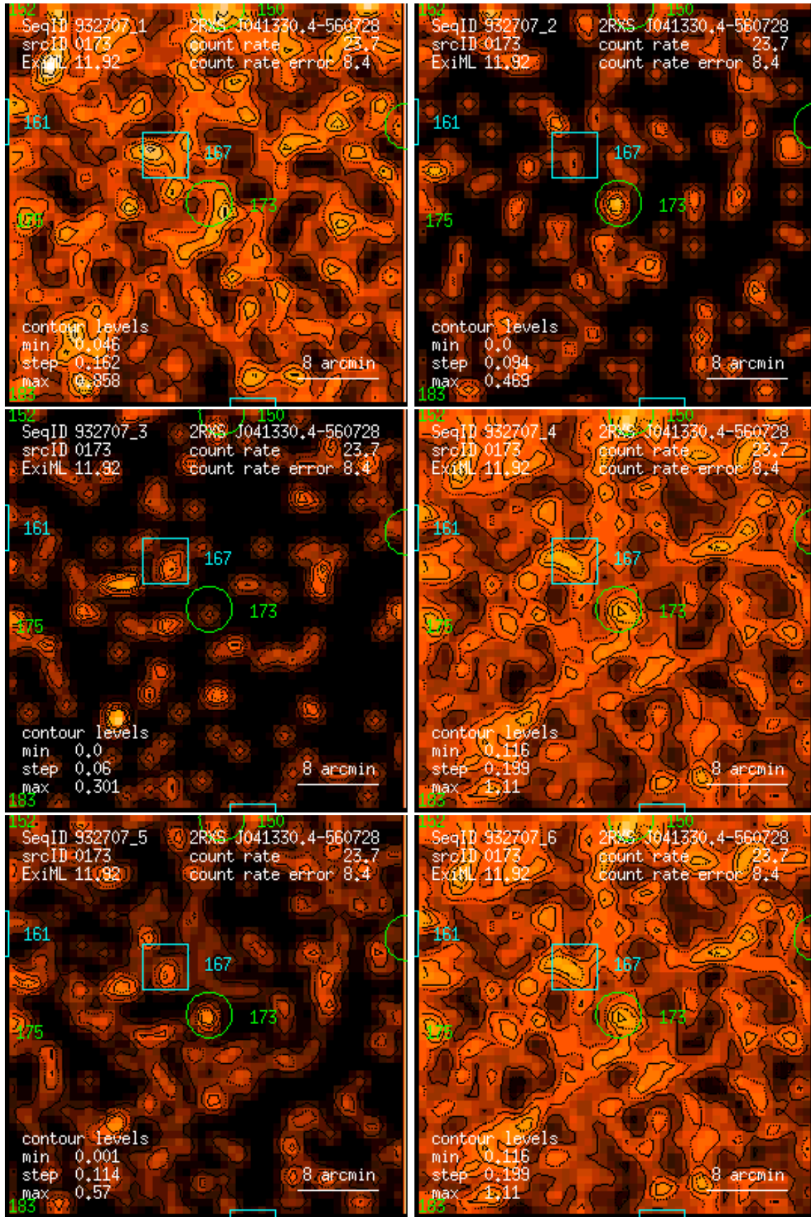
Figure 173: RASS 932707: detection 0173: band rate images, Gaussian filter: (1) PSPC channels 11 – 41, (2) 52 – 90, (3) 91 – 201, (4) 11 – 235, (5) 52 – 201, (6) 11 – 201. Broad band rates in counts/ks. Band rate contour levels in counts/ks/arcmin 2 .
