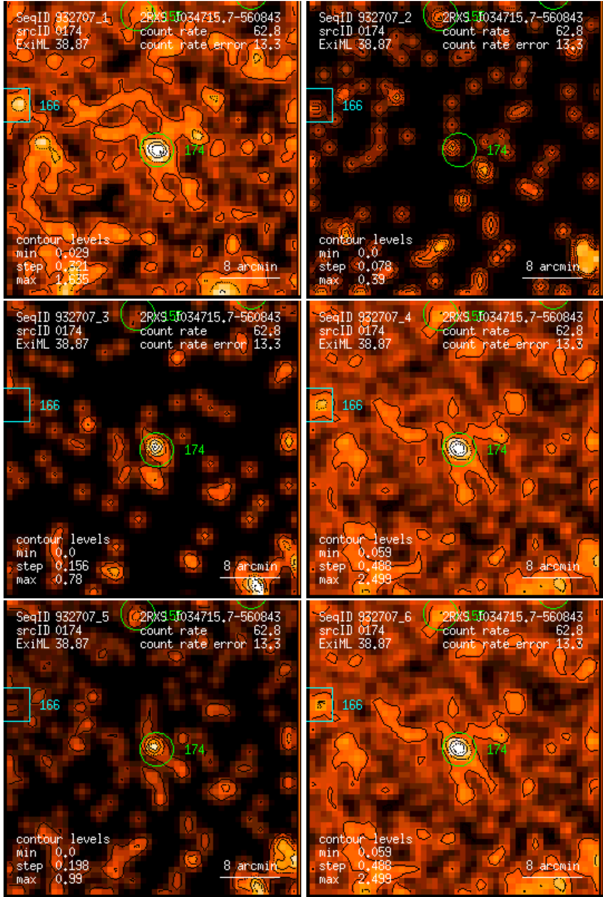
Figure 174: RASS 932707: detection 0174: band rate images, Gaussian filter: (1) PSPC channels 11 – 41, (2) 52 – 90, (3) 91 – 201, (4) 11 – 235, (5) 52 – 201, (6) 11 – 201. Broad band rates in counts/ks. Band rate contour levels in counts/ks/arcmin 2 .
