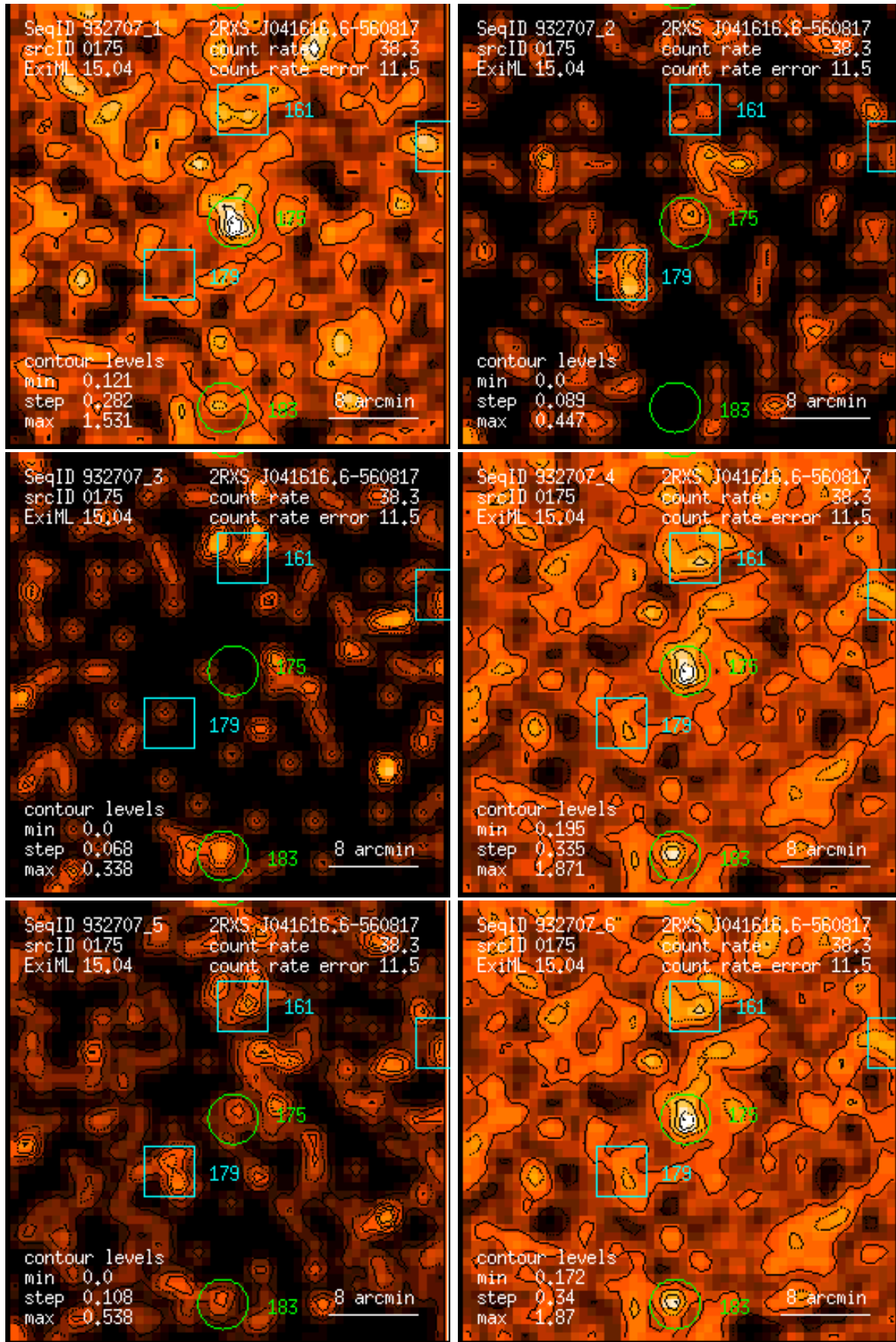
Figure 175: RASS 932707: detection 0175: band rate images, Gaussian filter: (1) PSPC channels 11 – 41, (2) 52 – 90, (3) 91 – 201, (4) 11 – 235, (5) 52 – 201, (6) 11 – 201. Broad band rates in counts/ks. Band rate contour levels in counts/ks/arcmin 2 .
