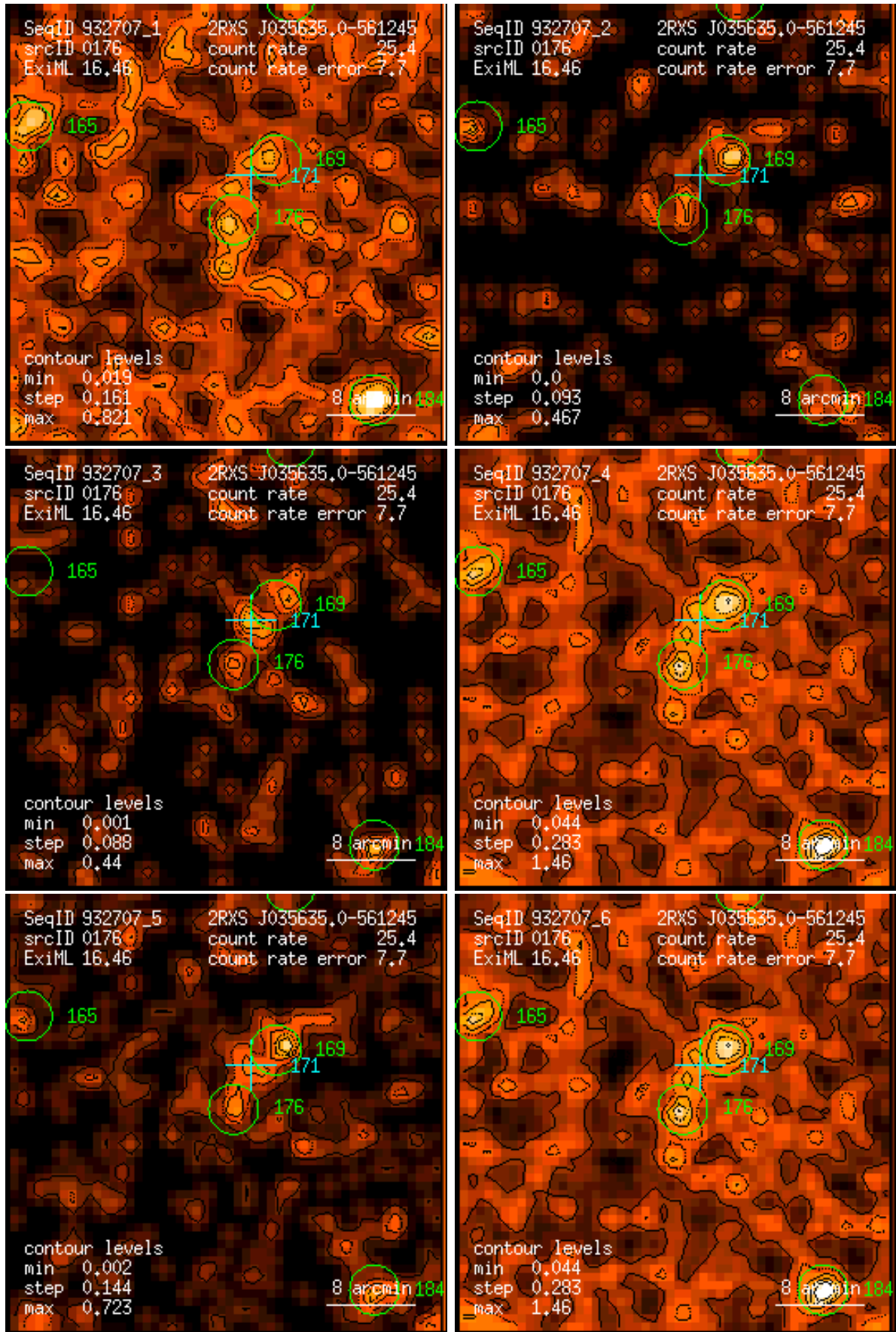
Figure 176: RASS 932707: detection 0176: band rate images, Gaussian filter: (1) PSPC channels 11 – 41, (2) 52 – 90, (3) 91 – 201, (4) 11 – 235, (5) 52 – 201, (6) 11 – 201. Broad band rates in counts/ks. Band rate contour levels in counts/ks/arcmin 2 .
