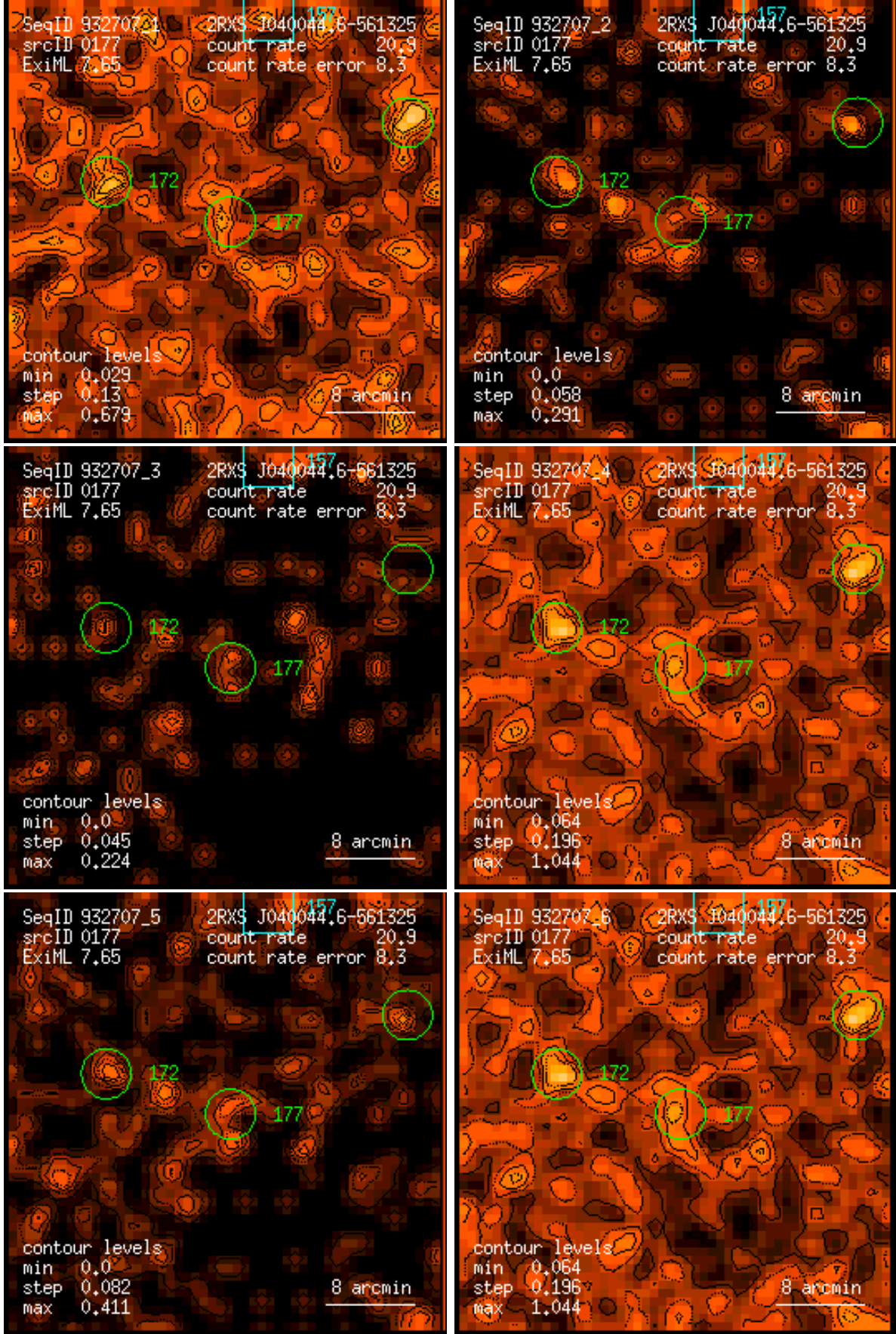
Figure 177: RASS 932707: detection 0177: band rate images, Gaussian filter: (1) PSPC channels 11 – 41, (2) 52 – 90, (3) 91 – 201, (4) 11 – 235, (5) 52 – 201, (6) 11 – 201. Broad band rates in counts/ks. Band rate contour levels in counts/ks/arcmin 2 .
