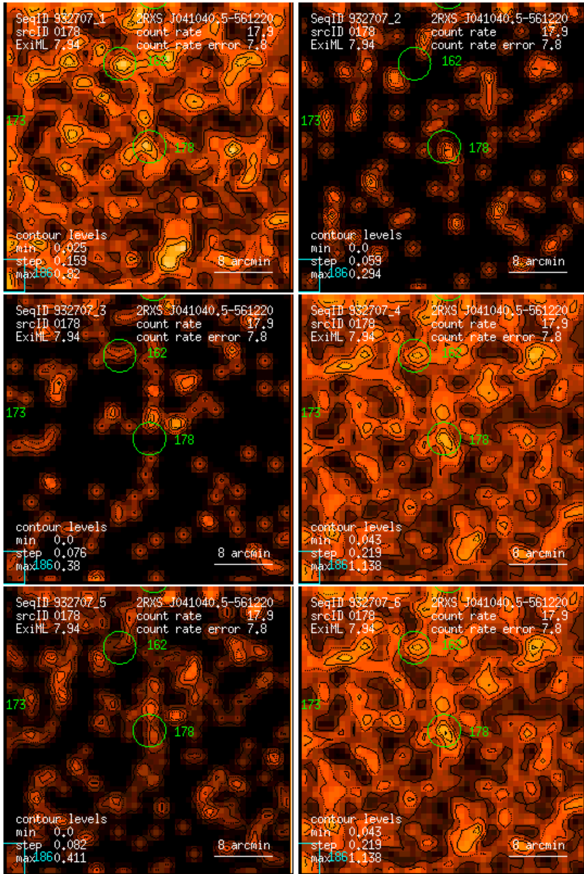
Figure 178: RASS 932707: detection 0178: band rate images, Gaussian filter: (1) PSPC channels 11 – 41, (2) 52 – 90, (3) 91 – 201, (4) 11 – 235, (5) 52 – 201, (6) 11 – 201. Broad band rates in counts/ks. Band rate contour levels in counts/ks/arcmin 2 .
