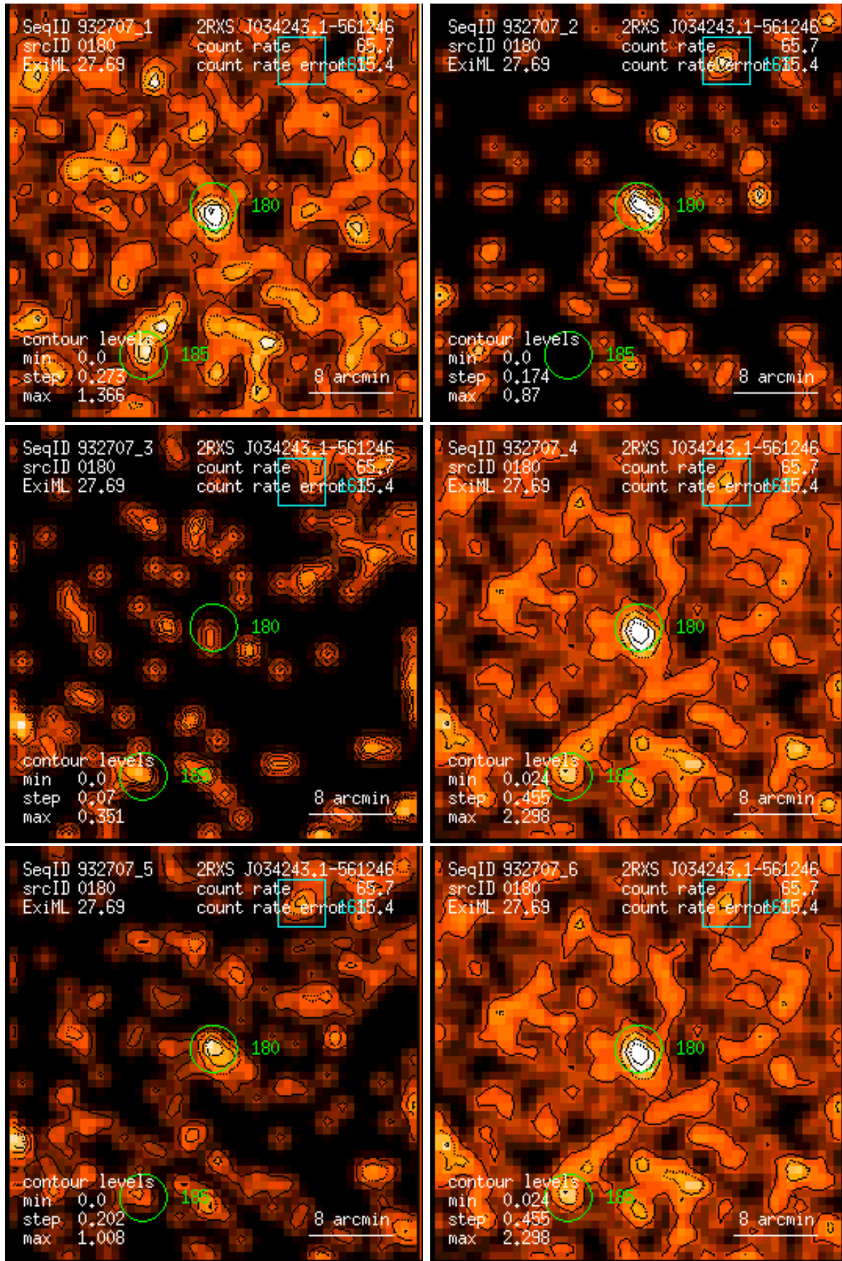
Figure 180: RASS 932707: detection 0180: band rate images, Gaussian filter: (1) PSPC channels 11 – 41, (2) 52 – 90, (3) 91 – 201, (4) 11 – 235, (5) 52 – 201, (6) 11 – 201. Broad band rates in counts/ks. Band rate contour levels in counts/ks/arcmin 2 .
