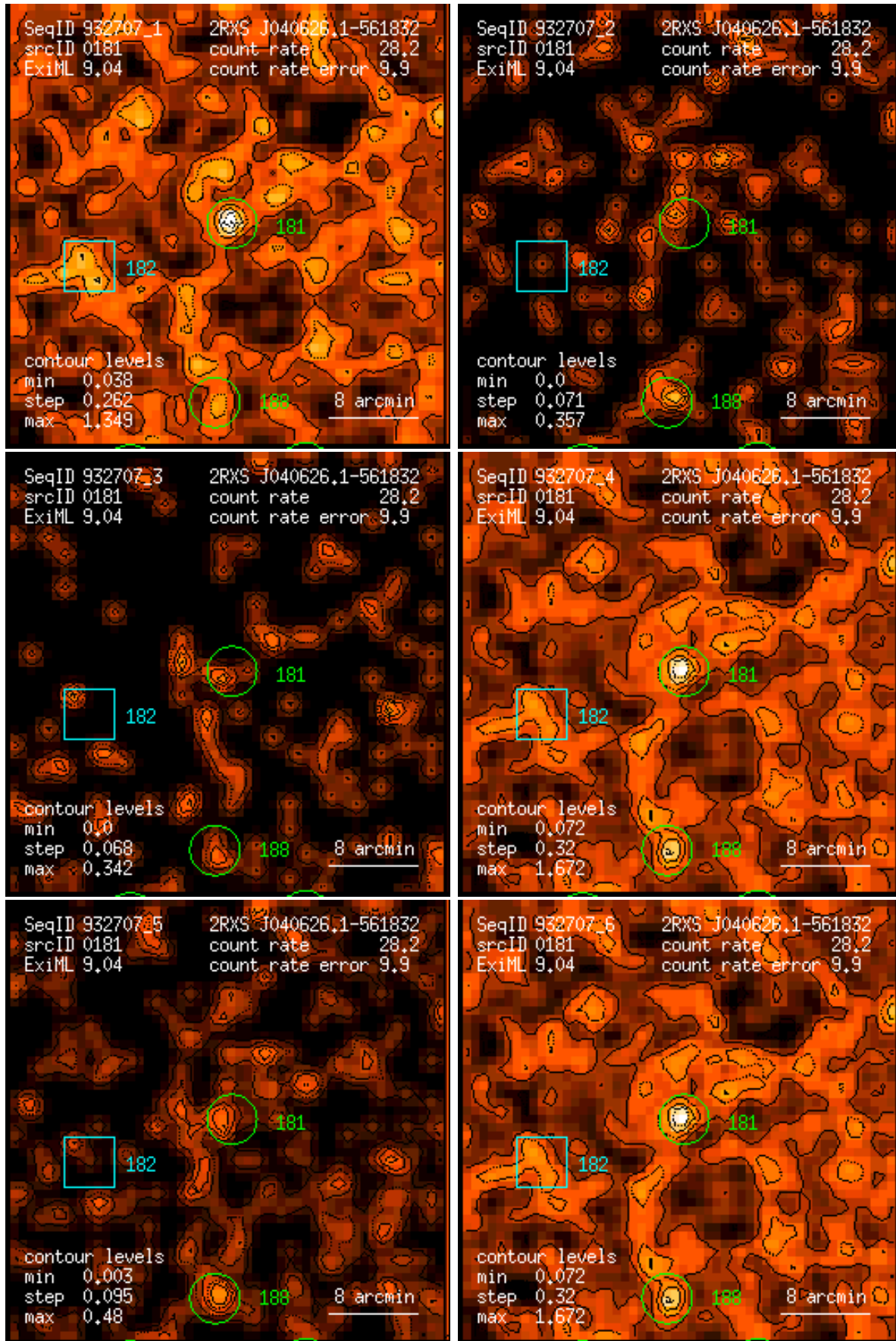
Figure 181: RASS 932707: detection 0181: band rate images, Gaussian filter: (1) PSPC channels 11 – 41, (2) 52 – 90, (3) 91 – 201, (4) 11 – 235, (5) 52 – 201, (6) 11 – 201. Broad band rates in counts/ks. Band rate contour levels in counts/ks/arcmin 2 .
