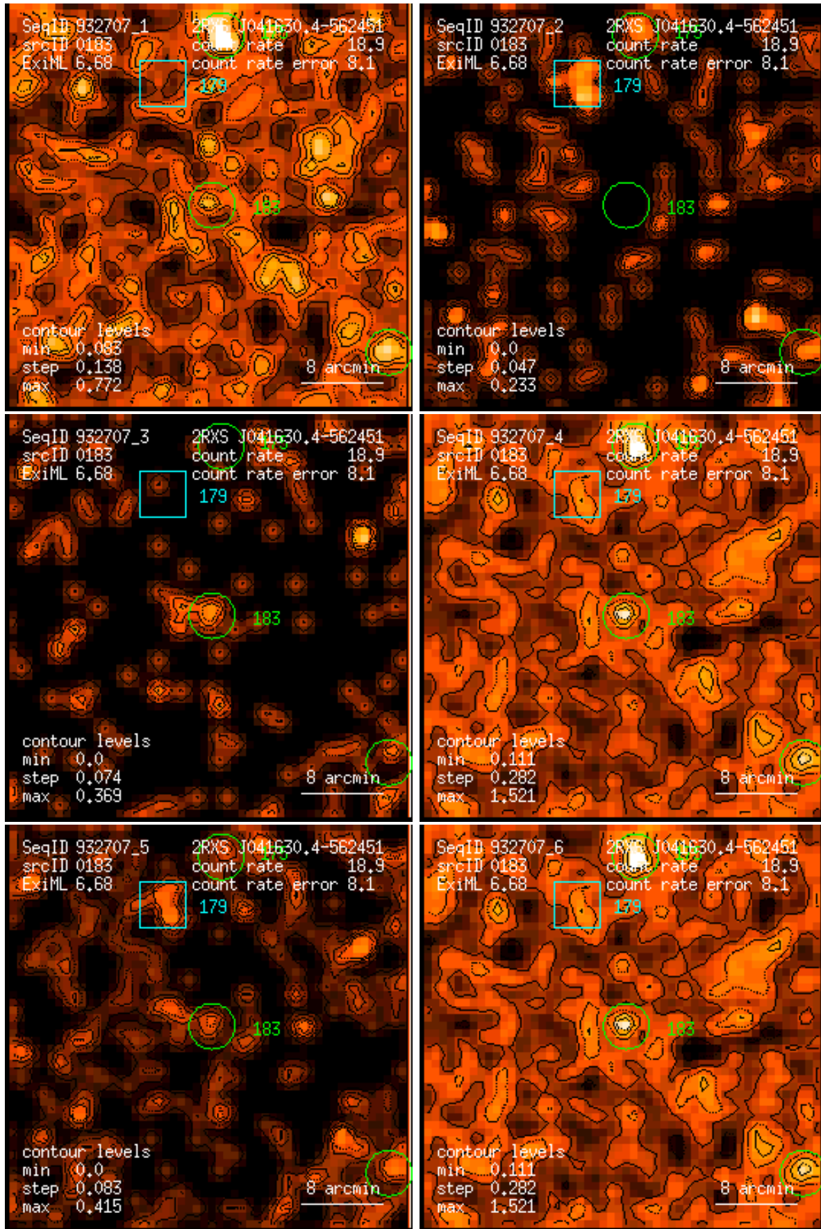
Figure 183: RASS 932707: detection 0183: band rate images, Gaussian filter: (1) PSPC channels 11 – 41, (2) 52 – 90, (3) 91 – 201, (4) 11 – 235, (5) 52 – 201, (6) 11 – 201. Broad band rates in counts/ks. Band rate contour levels in counts/ks/arcmin 2 .
