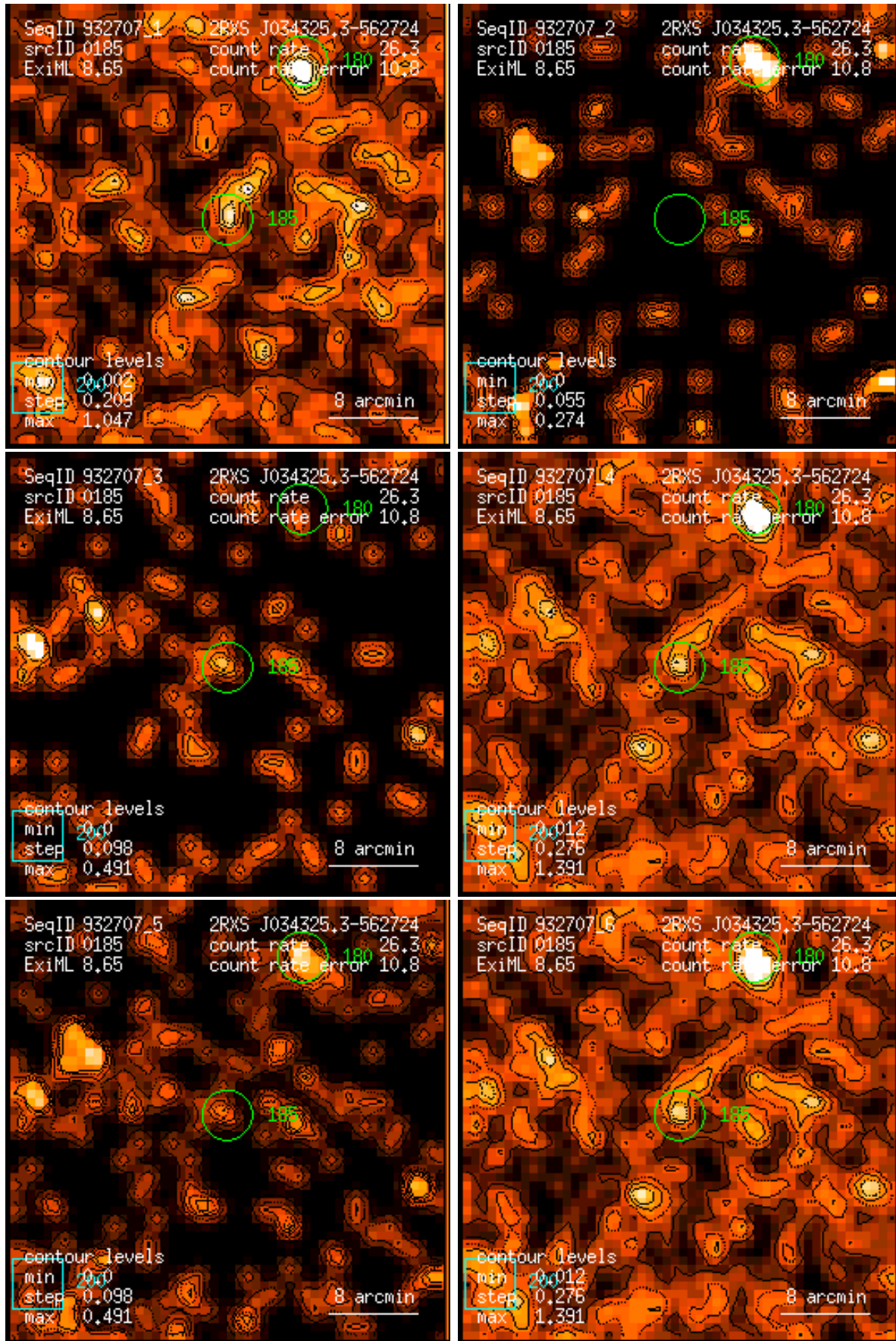
Figure 185: RASS 932707: detection 0185: band rate images, Gaussian filter: (1) PSPC channels 11 – 41, (2) 52 – 90, (3) 91 – 201, (4) 11 – 235, (5) 52 – 201, (6) 11 – 201. Broad band rates in counts/ks. Band rate contour levels in counts/ks/arcmin 2 .
