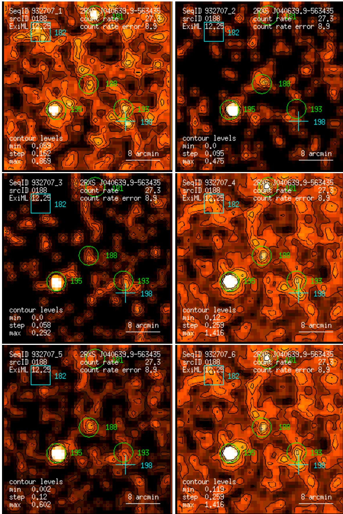
Figure 188: RASS 932707: detection 0188: band rate images, Gaussian filter: (1) PSPC channels 11 – 41, (2) 52 – 90, (3) 91 – 201, (4) 11 – 235, (5) 52 – 201, (6) 11 – 201. Broad band rates in counts/ks. Band rate contour levels in counts/ks/arcmin 2 .
