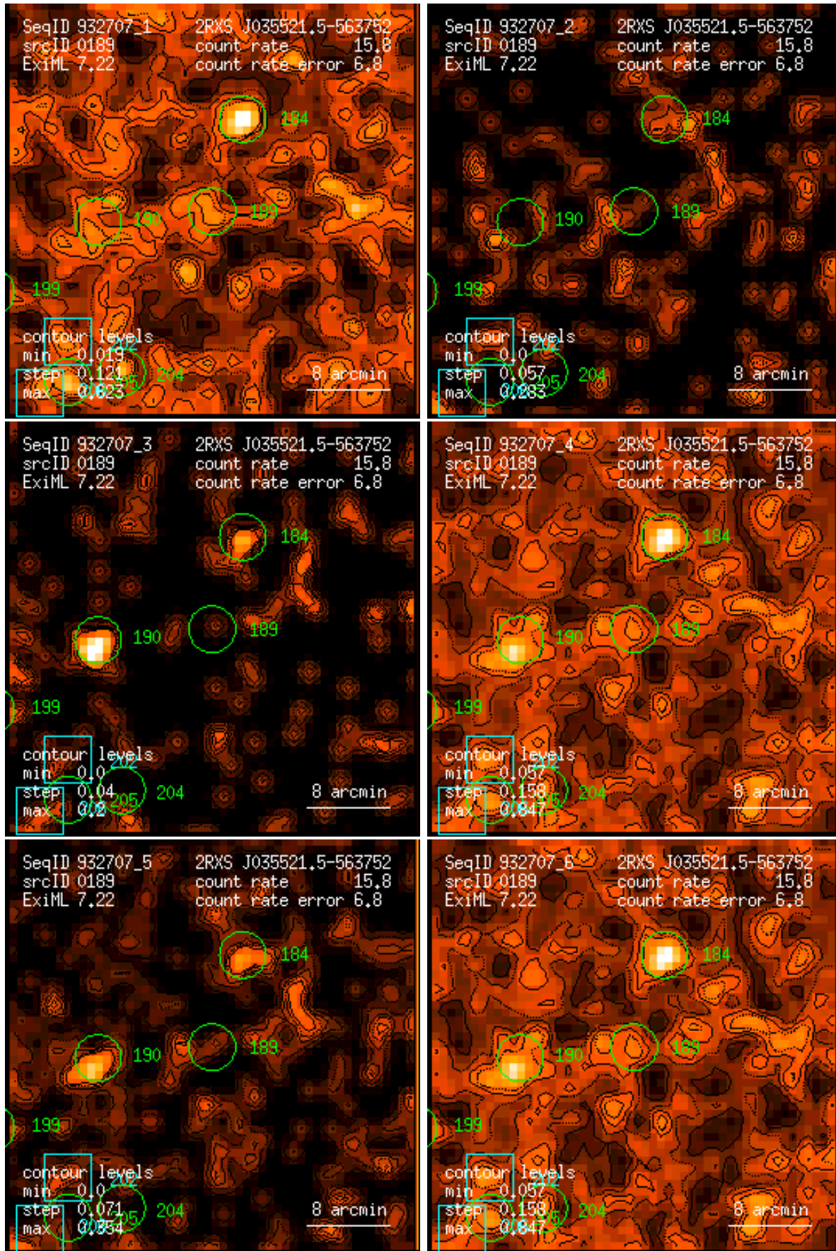
Figure 189: RASS 932707: detection 0189: band rate images, Gaussian filter: (1) PSPC channels 11 – 41, (2) 52 – 90, (3) 91 – 201, (4) 11 – 235, (5) 52 – 201, (6) 11 – 201. Broad band rates in counts/ks. Band rate contour levels in counts/ks/arcmin 2 .
