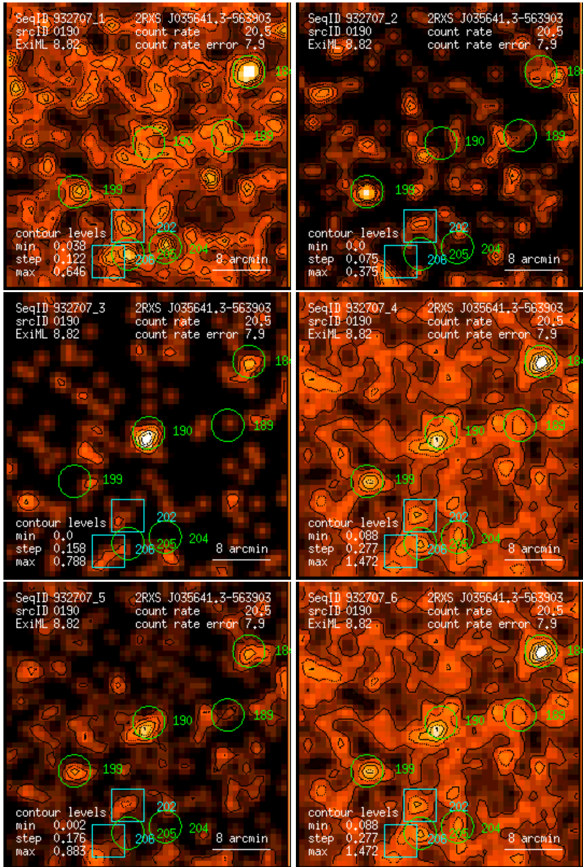
Figure 190: RASS 932707: detection 0190: band rate images, Gaussian filter: (1) PSPC channels 11 – 41, (2) 52 – 90, (3) 91 – 201, (4) 11 – 235, (5) 52 – 201, (6) 11 – 201. Broad band rates in counts/ks. Band rate contour levels in counts/ks/arcmin 2 .
