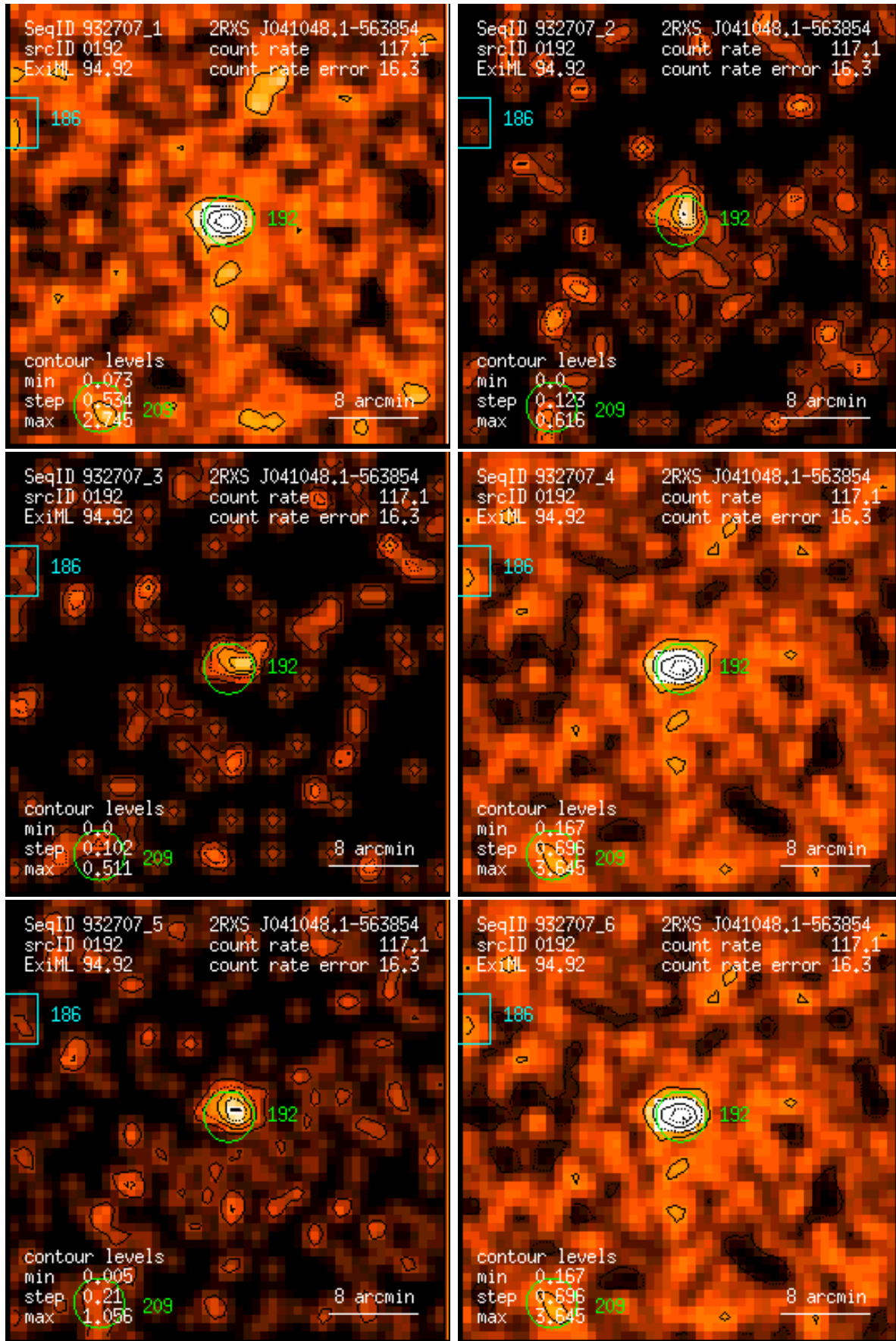
Figure 192: RASS 932707: detection 0192: band rate images, Gaussian filter: (1) PSPC channels 11 – 41, (2) 52 – 90, (3) 91 – 201, (4) 11 – 235, (5) 52 – 201, (6) 11 – 201. Broad band rates in counts/ks. Band rate contour levels in counts/ks/arcmin 2 .
