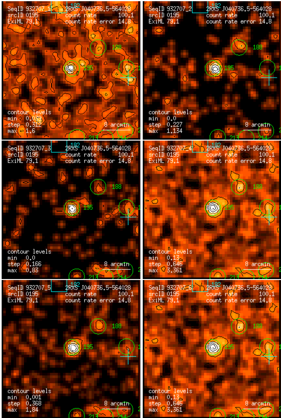
Figure 195: RASS 932707: detection 0195: band rate images, Gaussian filter: (1) PSPC channels 11 – 41, (2) 52 – 90, (3) 91 – 201, (4) 11 – 235, (5) 52 – 201, (6) 11 – 201. Broad band rates in counts/ks. Band rate contour levels in counts/ks/arcmin 2 .
