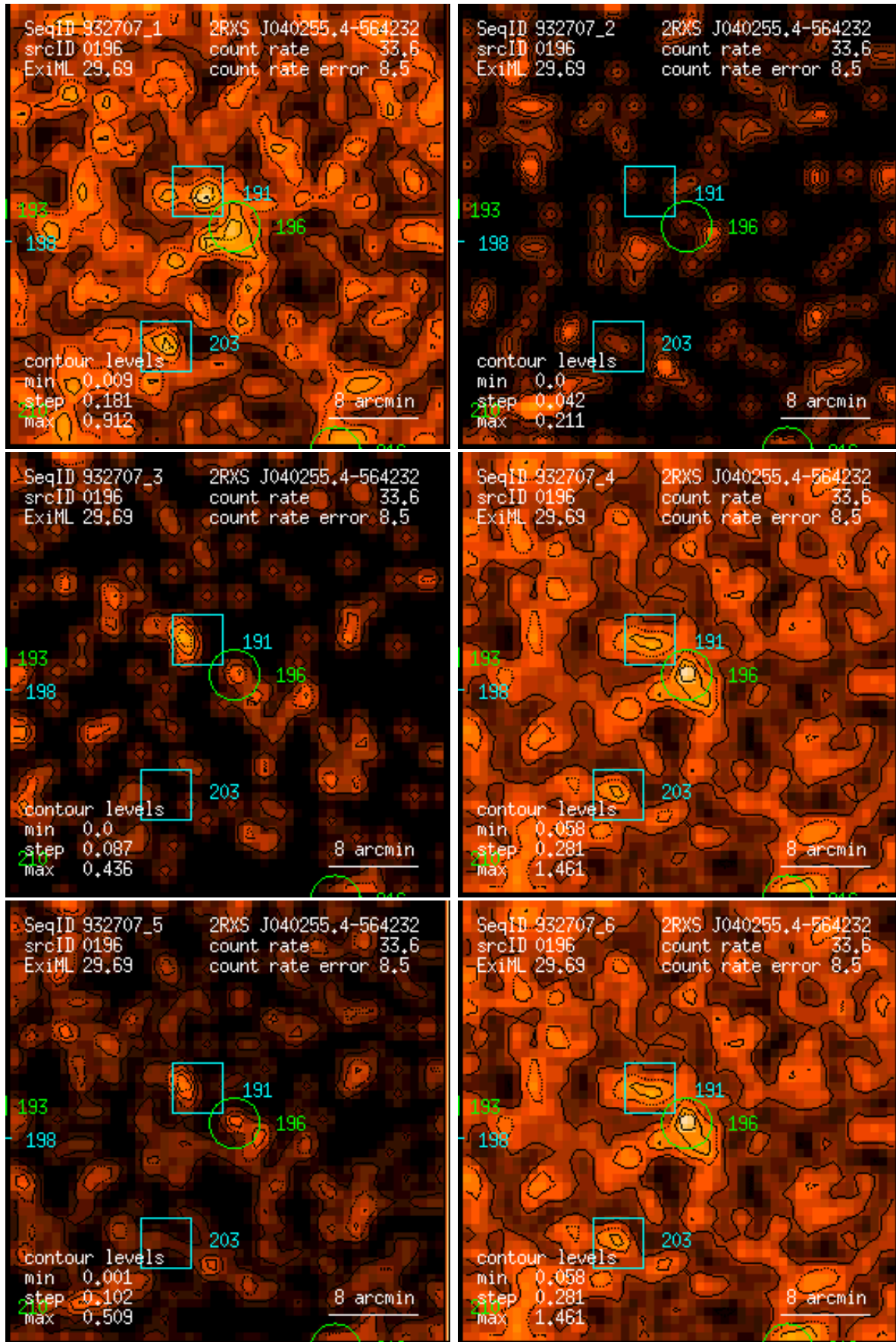
Figure 196: RASS 932707: detection 0196: band rate images, Gaussian filter: (1) PSPC channels 11 – 41, (2) 52 – 90, (3) 91 – 201, (4) 11 – 235, (5) 52 – 201, (6) 11 – 201. Broad band rates in counts/ks. Band rate contour levels in counts/ks/arcmin 2 .
