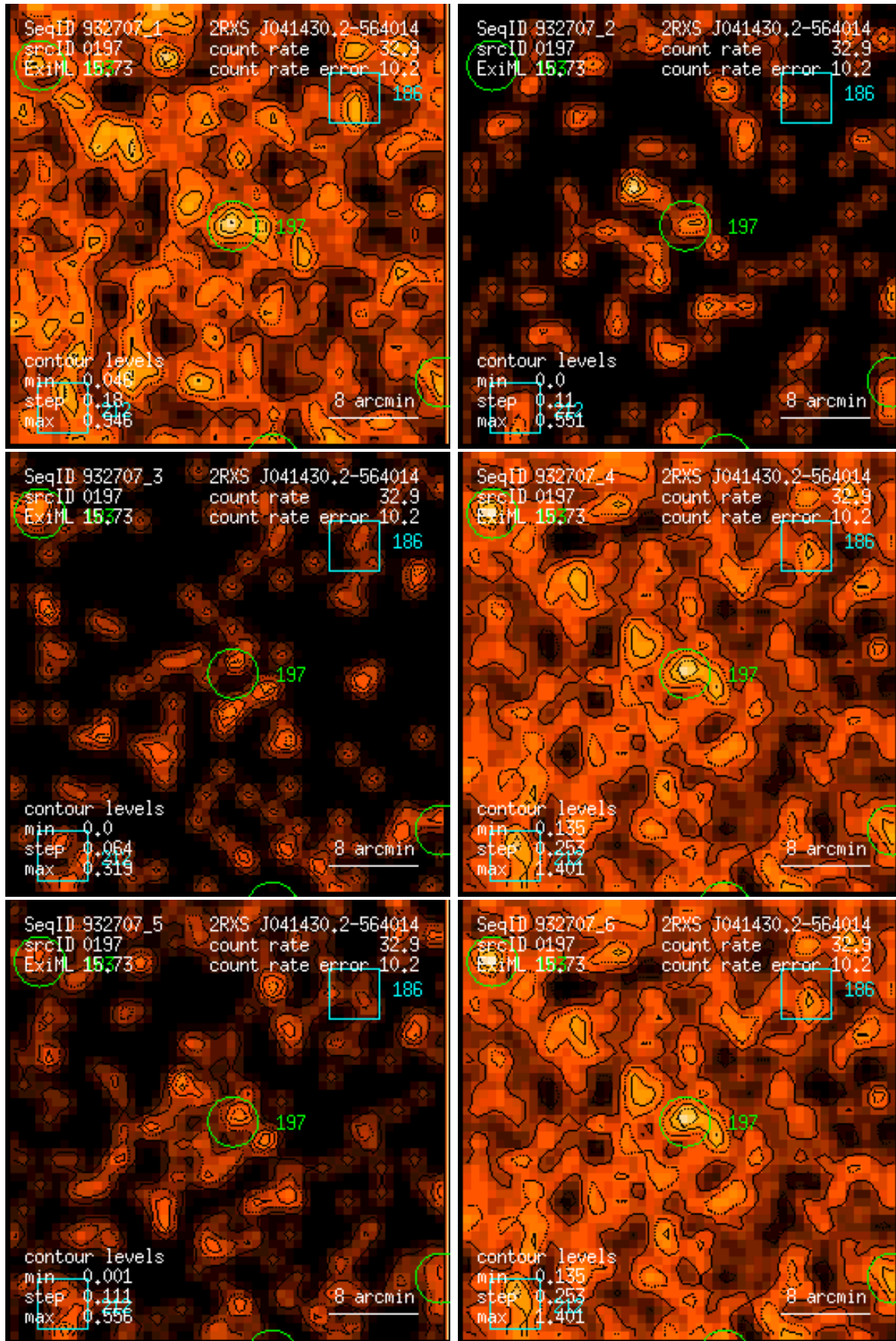
Figure 197: RASS 932707: detection 0197: band rate images, Gaussian filter: (1) PSPC channels 11 – 41, (2) 52 – 90, (3) 91 – 201, (4) 11 – 235, (5) 52 – 201, (6) 11 – 201. Broad band rates in counts/ks. Band rate contour levels in counts/ks/arcmin 2 .
