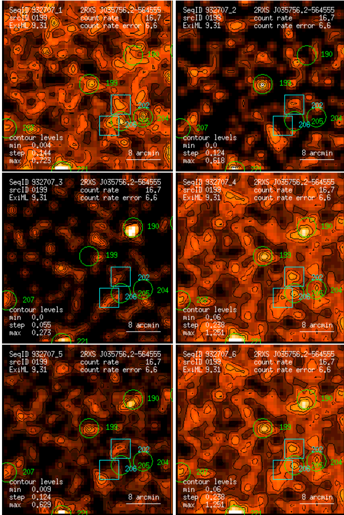
Figure 199: RASS 932707: detection 0199: band rate images, Gaussian filter: (1) PSPC channels 11 – 41, (2) 52 – 90, (3) 91 – 201, (4) 11 – 235, (5) 52 – 201, (6) 11 – 201. Broad band rates in counts/ks. Band rate contour levels in counts/ks/arcmin 2 .
