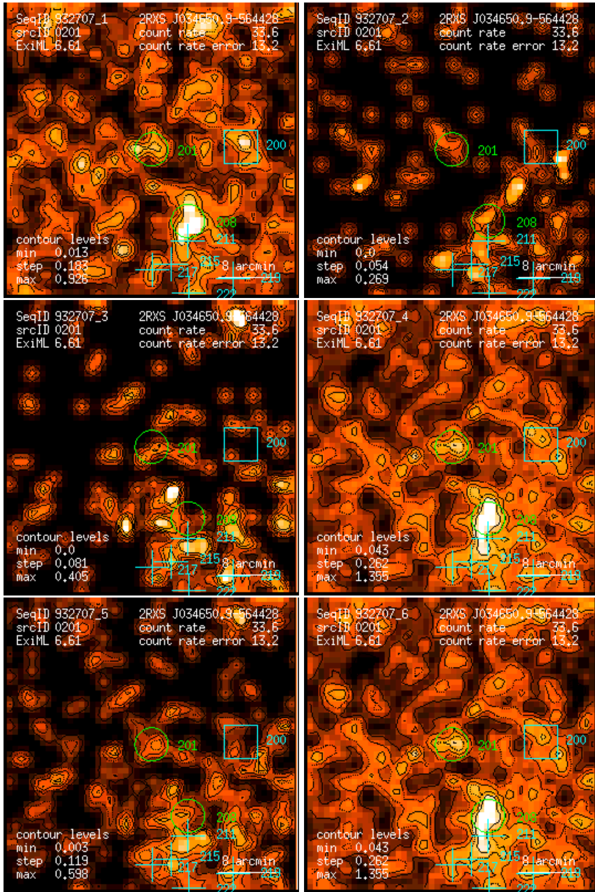
Figure 201: RASS 932707: detection 0201: band rate images, Gaussian filter: (1) PSPC channels 11 – 41, (2) 52 – 90, (3) 91 – 201, (4) 11 – 235, (5) 52 – 201, (6) 11 – 201. Broad band rates in counts/ks. Band rate contour levels in counts/ks/arcmin 2 .
