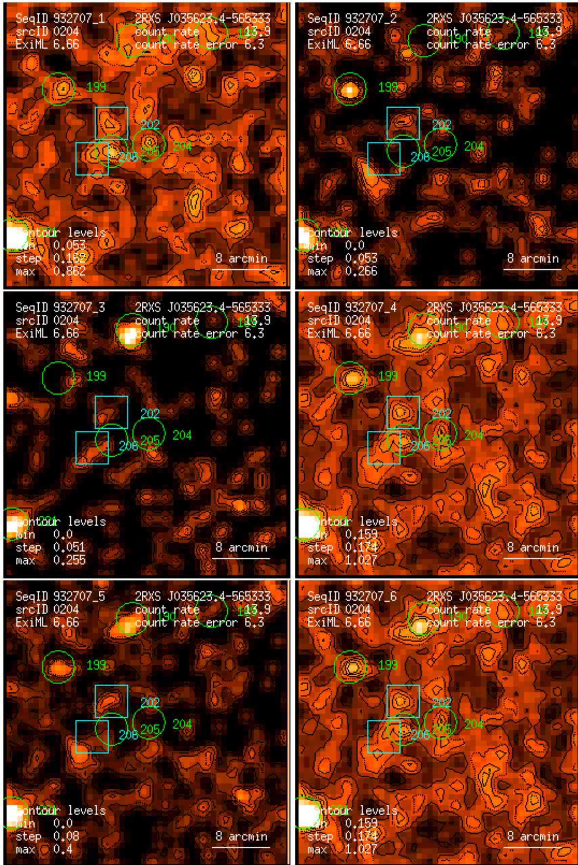
Figure 204: RASS 932707: detection 0204: band rate images, Gaussian filter: (1) PSPC channels 11 – 41, (2) 52 – 90, (3) 91 – 201, (4) 11 – 235, (5) 52 – 201, (6) 11 – 201. Broad band rates in counts/ks. Band rate contour levels in counts/ks/arcmin 2 .
