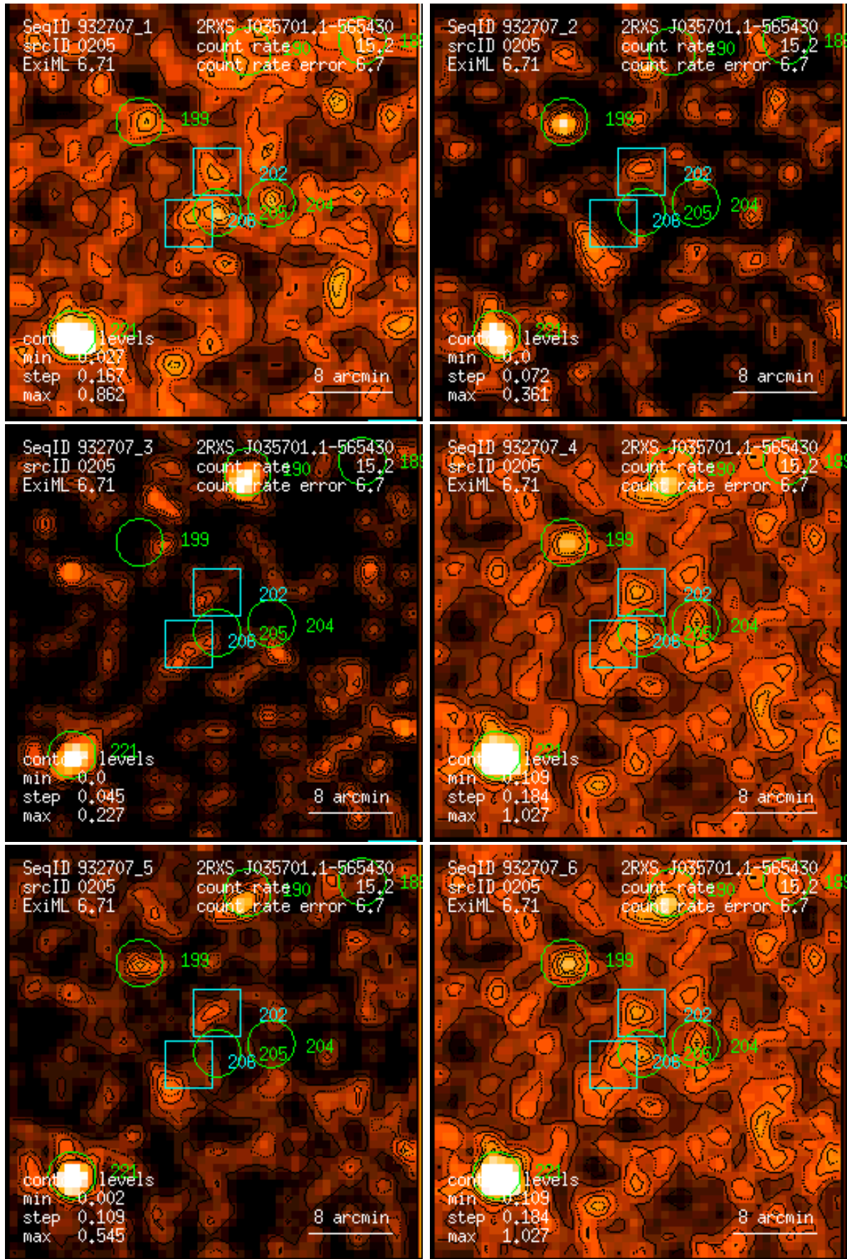
Figure 205: RASS 932707: detection 0205: band rate images, Gaussian filter: (1) PSPC channels 11 – 41, (2) 52 – 90, (3) 91 – 201, (4) 11 – 235, (5) 52 – 201, (6) 11 – 201. Broad band rates in counts/ks. Band rate contour levels in counts/ks/arcmin 2 .
