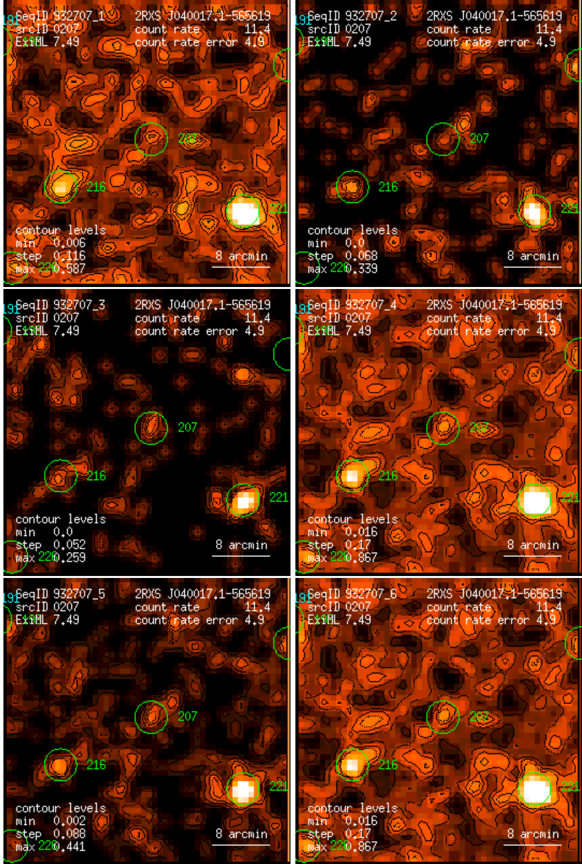
Figure 207: RASS 932707: detection 0207: band rate images, Gaussian filter: (1) PSPC channels 11 – 41, (2) 52 – 90, (3) 91 – 201, (4) 11 – 235, (5) 52 – 201, (6) 11 – 201. Broad band rates in counts/ks. Band rate contour levels in counts/ks/arcmin 2 .
