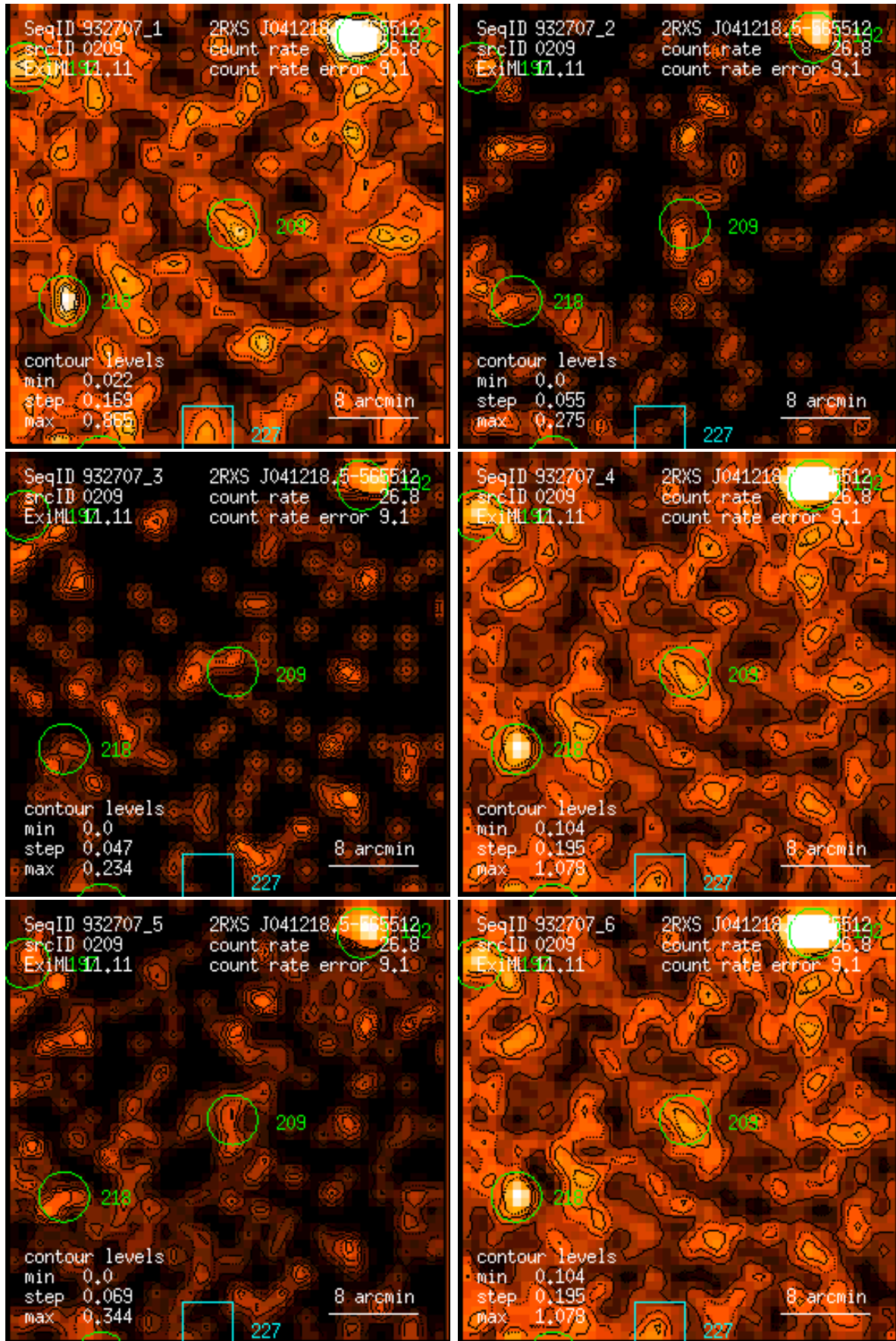
Figure 209: RASS 932707: detection 0209: band rate images, Gaussian filter: (1) PSPC channels 11 – 41, (2) 52 – 90, (3) 91 – 201, (4) 11 – 235, (5) 52 – 201, (6) 11 – 201. Broad band rates in counts/ks. Band rate contour levels in counts/ks/arcmin 2 .
