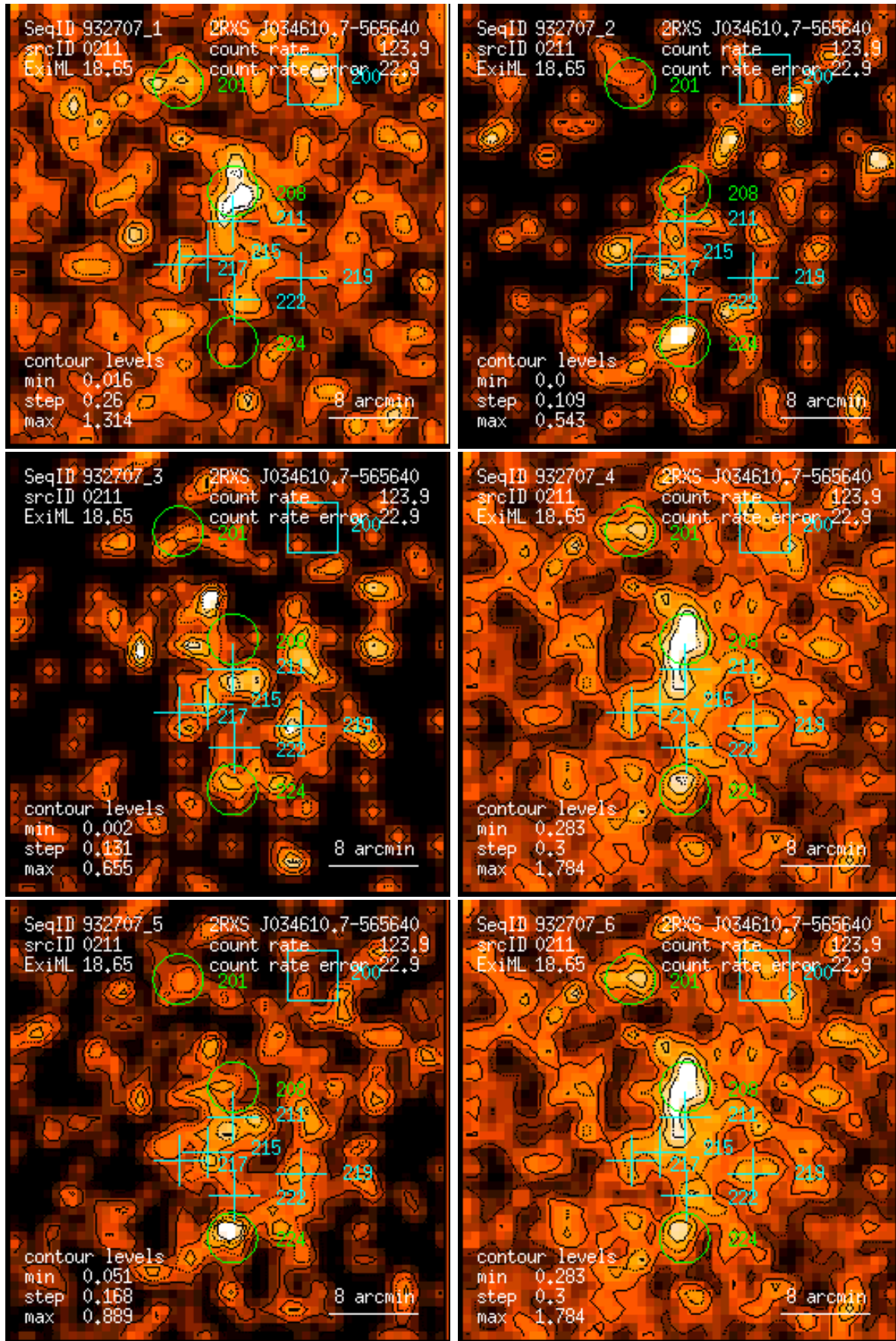
Figure 211: RASS 932707: detection 0211: band rate images, Gaussian filter: (1) PSPC channels 11 – 41, (2) 52 – 90, (3) 91 – 201, (4) 11 – 235, (5) 52 – 201, (6) 11 – 201. Broad band rates in counts/ks. Band rate contour levels in counts/ks/arcmin 2 .
