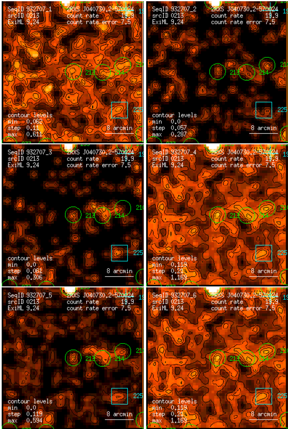
Figure 213: RASS 932707: detection 0213: band rate images, Gaussian filter: (1) PSPC channels 11 – 41, (2) 52 – 90, (3) 91 – 201, (4) 11 – 235, (5) 52 – 201, (6) 11 – 201. Broad band rates in counts/ks. Band rate contour levels in counts/ks/arcmin 2 .
