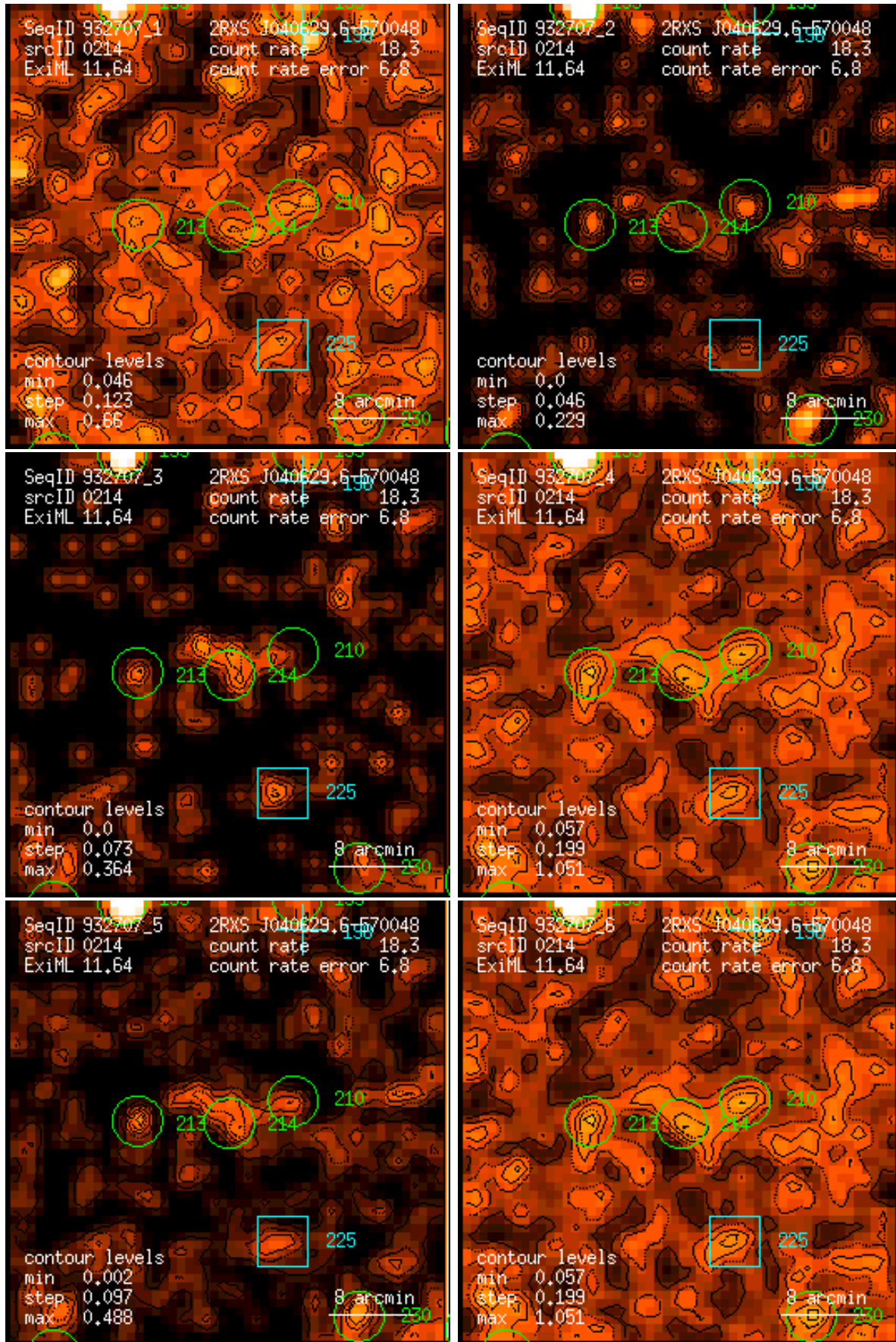
Figure 214: RASS 932707: detection 0214: band rate images, Gaussian filter: (1) PSPC channels 11 – 41, (2) 52 – 90, (3) 91 – 201, (4) 11 – 235, (5) 52 – 201, (6) 11 – 201. Broad band rates in counts/ks. Band rate contour levels in counts/ks/arcmin 2 .
