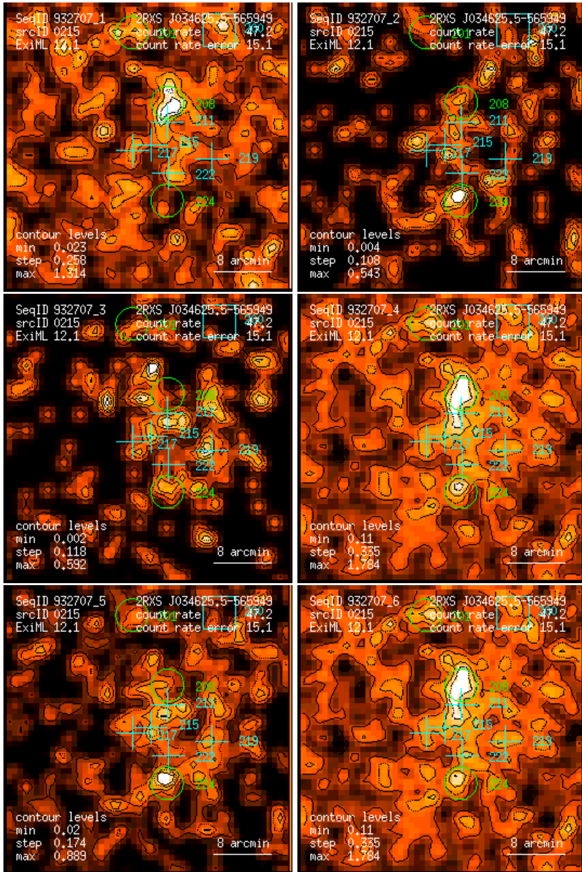
Figure 215: RASS 932707: detection 0215: band rate images, Gaussian filter: (1) PSPC channels 11 – 41, (2) 52 – 90, (3) 91 – 201, (4) 11 – 235, (5) 52 – 201, (6) 11 – 201. Broad band rates in counts/ks. Band rate contour levels in counts/ks/arcmin 2 .
