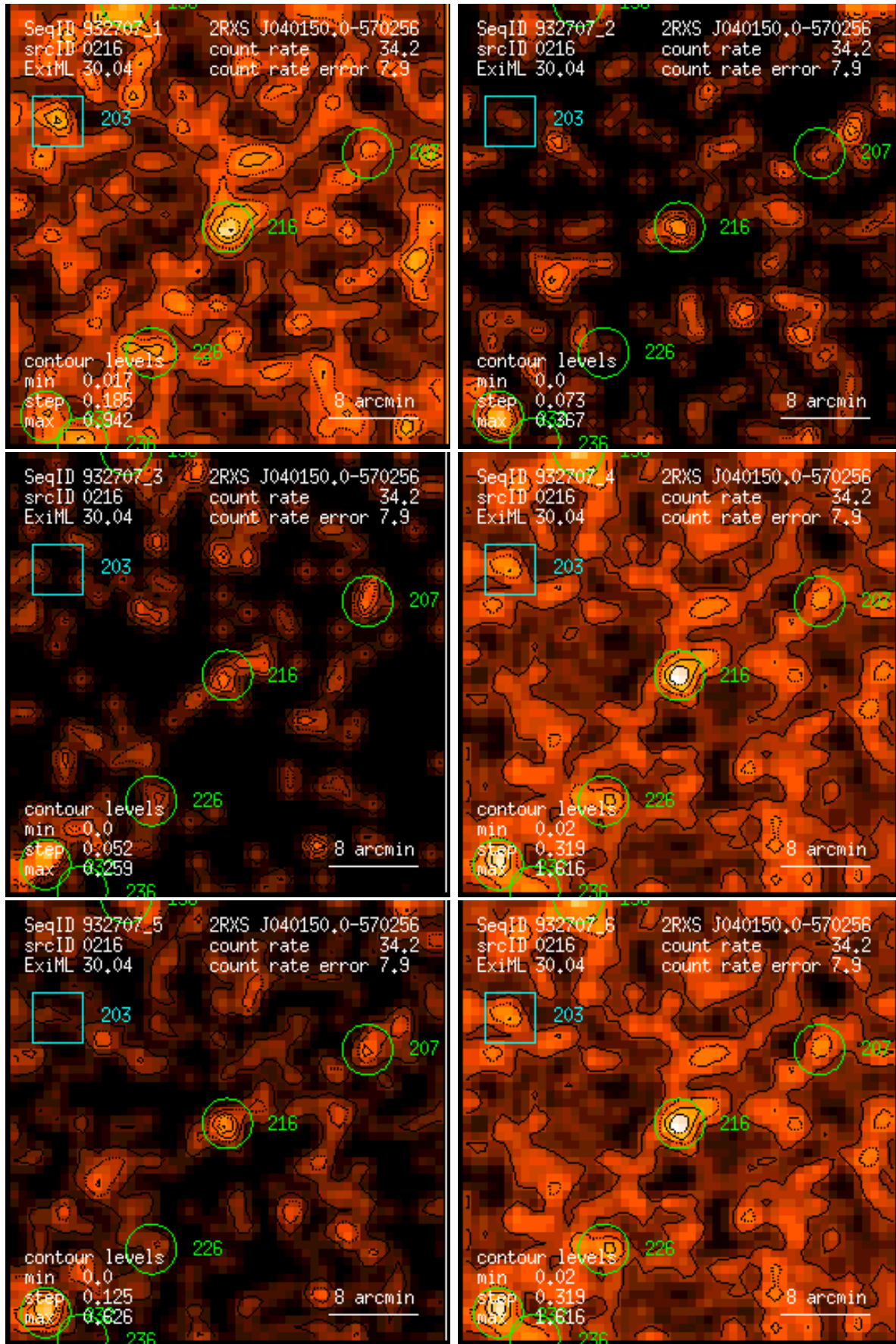
Figure 216: RASS 932707: detection 0216: band rate images, Gaussian filter: (1) PSPC channels 11 – 41, (2) 52 – 90, (3) 91 – 201, (4) 11 – 235, (5) 52 – 201, (6) 11 – 201. Broad band rates in counts/ks. Band rate contour levels in counts/ks/arcmin 2 .
